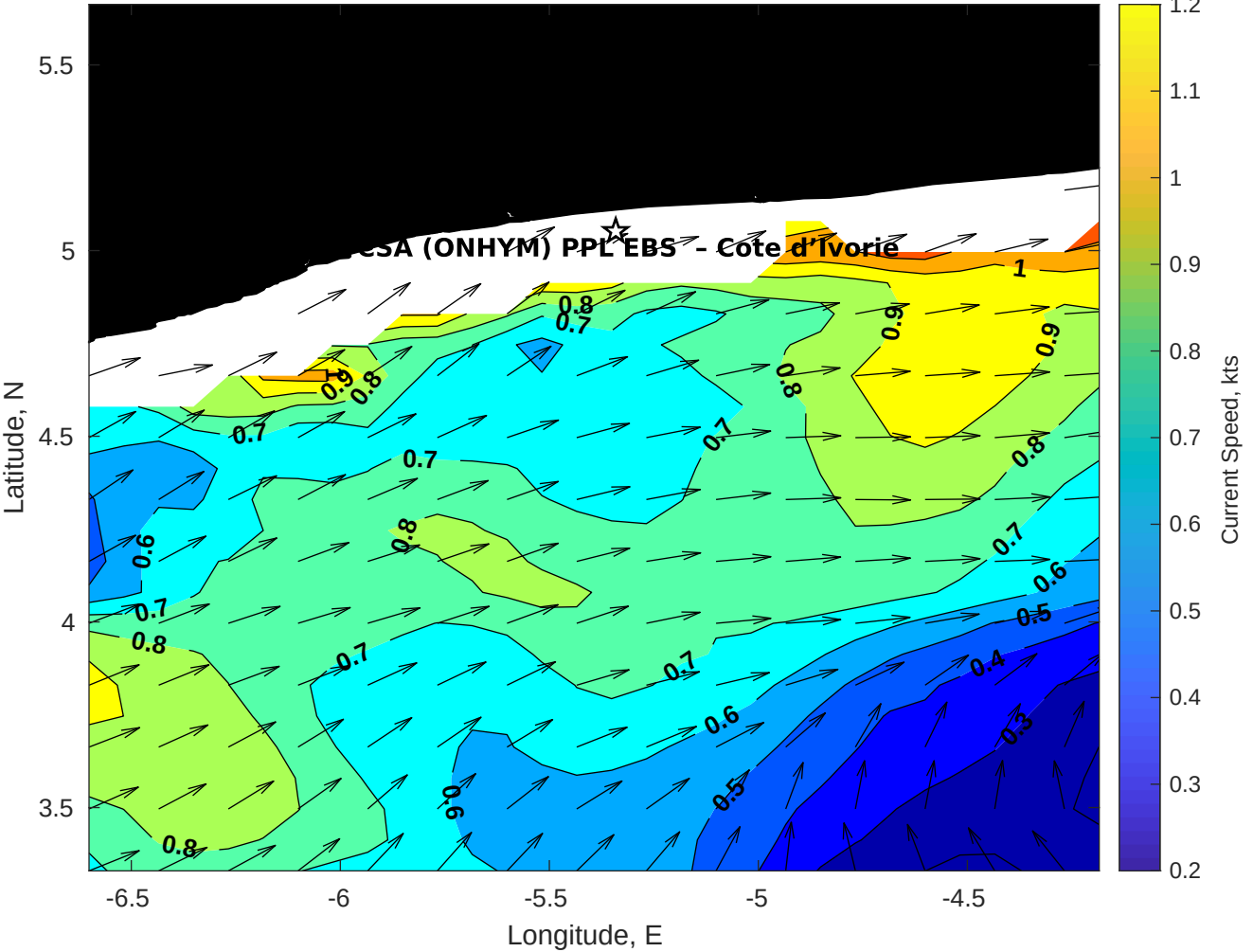
Surface Currents for CSA (ONHYM) PPL EBS - Cote d'Ivoire at 10-Dec-2025 00:00:00
