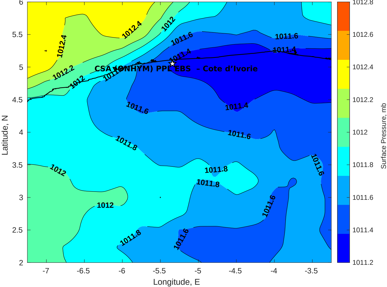
Surface Pressure (mb) for CSA (ONHYM) PPL EBS - Cote d'Ivoire at 12-Dec-2025 00:00:00
