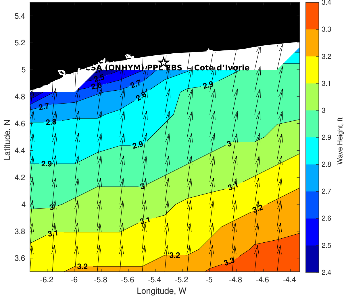
GFS Wave Height (ft) for CSA (ONHYM) PPL EBS - Cote d'Ivoire at 11-Dec-2025 09:00:00
