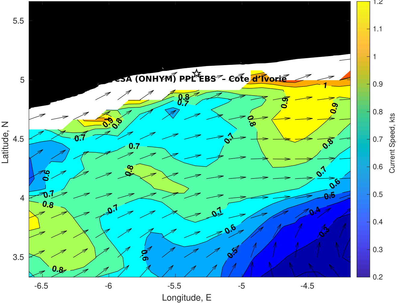
Surface Currents for CSA (ONHYM) PPL EBS - Cote d'Ivoire at 10-Dec-2025 00:00:00
