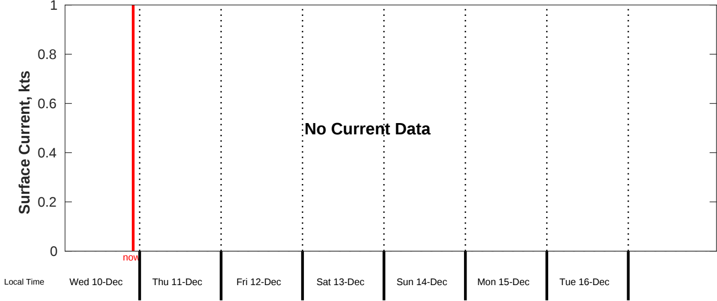
Surface Current Forecast for CSA (ONHYM) PPL EBS - Cote d'Ivoire from 10-Dec-2025 00:00:00 to 18-Dec-2025 00:00:00
