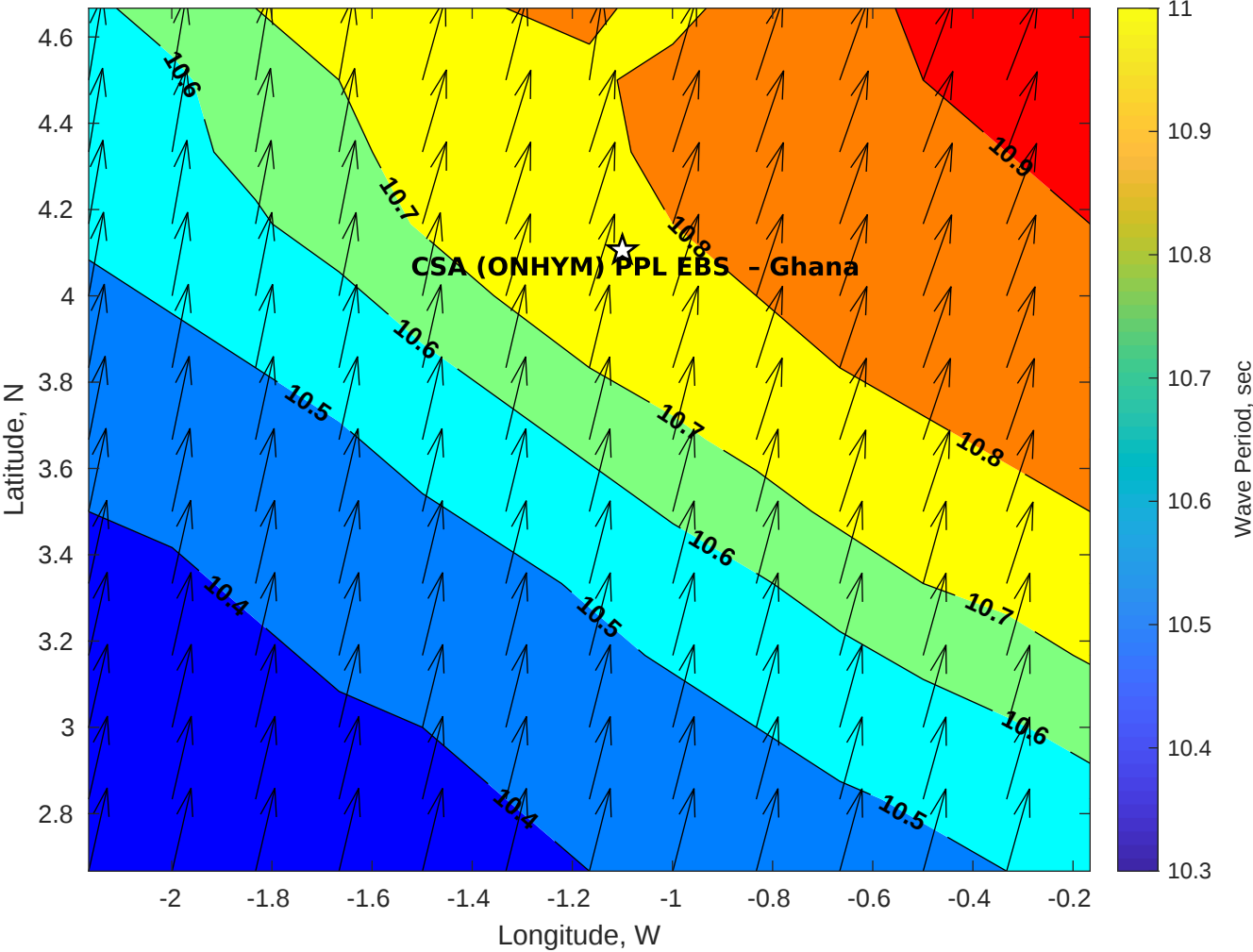
GFS Wave Period (sec) for CSA (ONHYM) PPL EBS - Ghana at 11-Dec-2025 09:00:00
