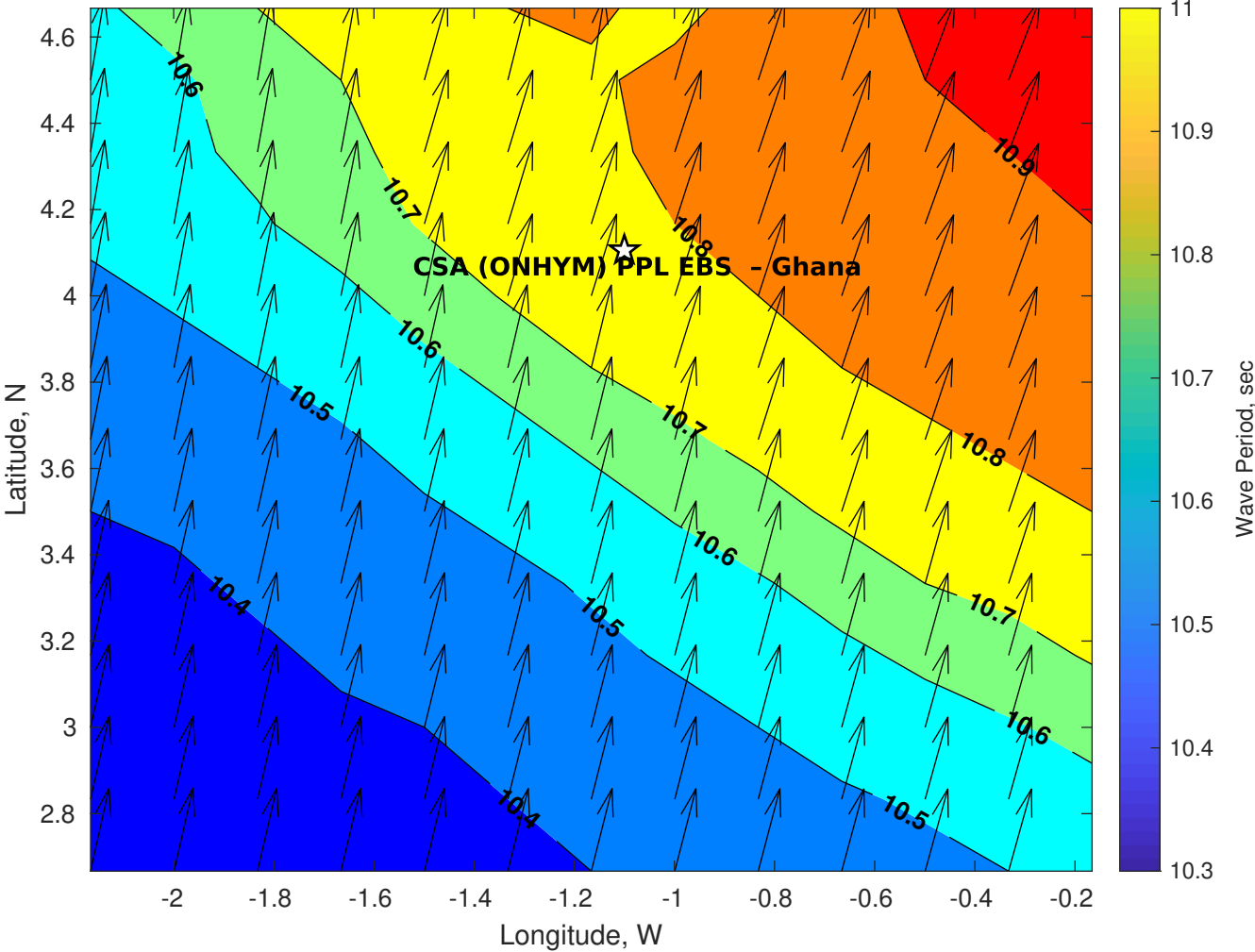
GFS Wave Period (sec) for CSA (ONHYM) PPL EBS - Ghana at 11-Dec-2025 09:00:00
