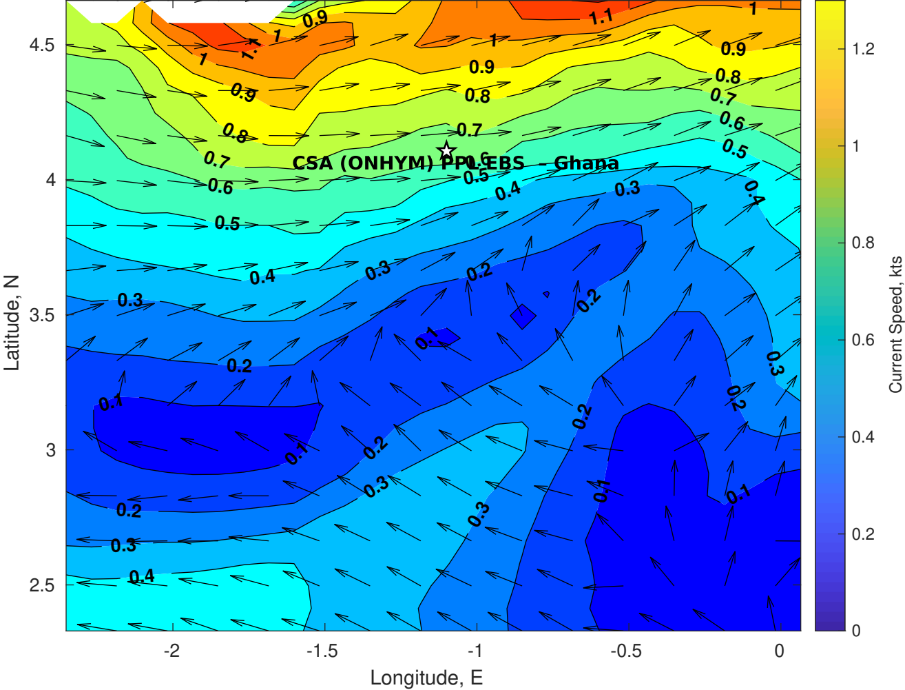
Surface Currents for CSA (ONHYM) PPL EBS - Ghana at 10-Dec-2025 00:00:00
