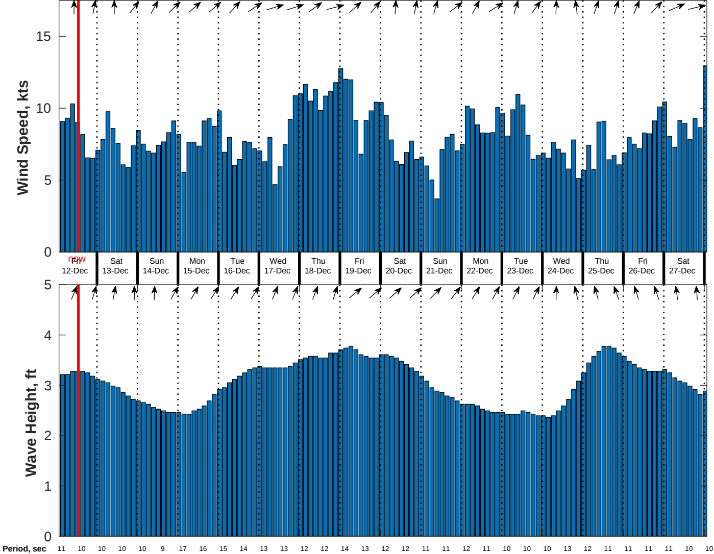
Wind & Wave Forecast for CSA (ONHYM) PPL EBS - Ghana from 11-Dec-2025 02:00:00 to 27-Dec-2025 02:00:00
