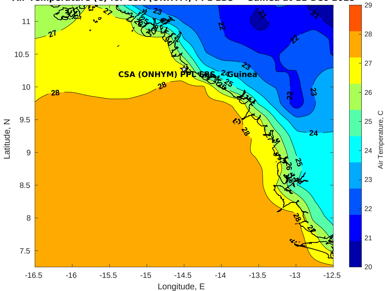
Air Temperature (C) for CSA (ONHYM) PPL EBS - Guinea at 11-Dec-2025
