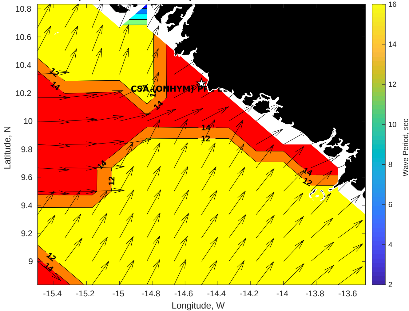
GFS Wave Period (sec) for CSA (ONHYM) PPL EBS - Guinea at 11-Dec-2025 09:00:00
