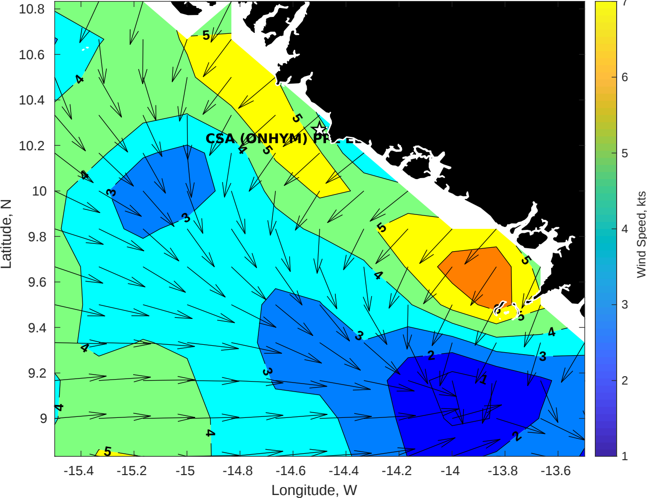
GFS Winds (kts) for CSA (ONHYM) PPL EBS - Guinea at 11-Dec-2025 09:00:00
