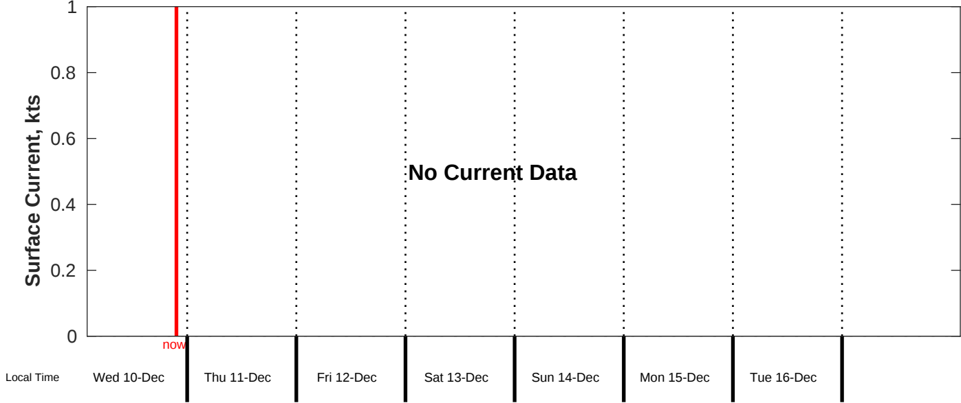
Surface Current Forecast for CSA (ONHYM) PPL EBS - Guinea from 10-Dec-2025 00:00:00 to 18-Dec-2025 00:00:00
