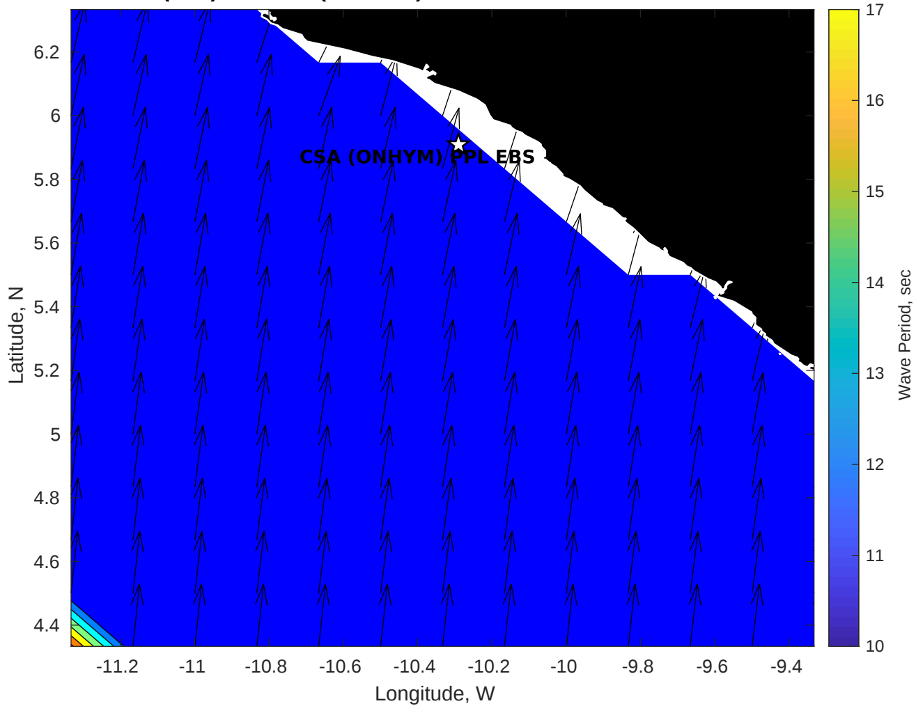
GFS Wave Period (sec) for CSA (ONHYM) PPL EBS - Liberia at 11-Dec-2025 09:00:00
