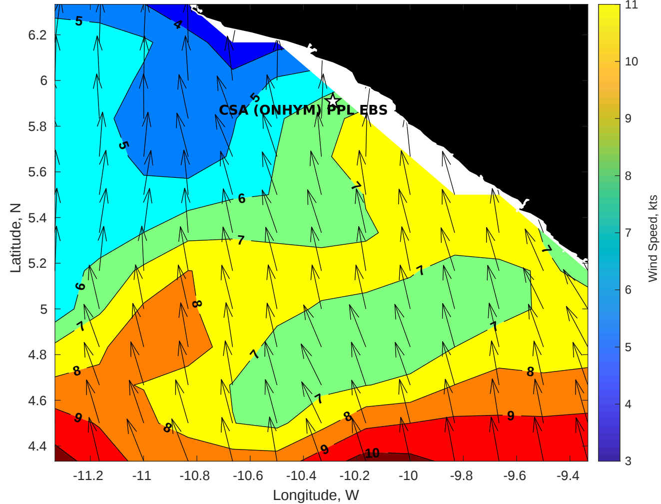
GFS Winds (kts) for CSA (ONHYM) PPL EBS - Liberia at 11-Dec-2025 09:00:00
