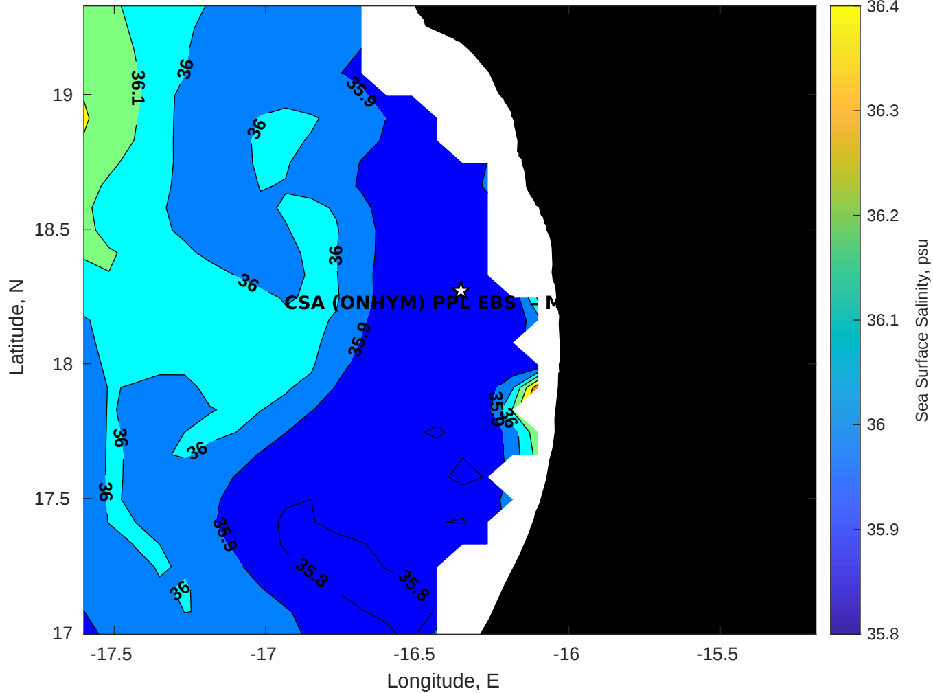
Surface Salinity for CSA (ONHYM) PPL EBS - Mauritania at 10-Dec-2025 00:00:00
