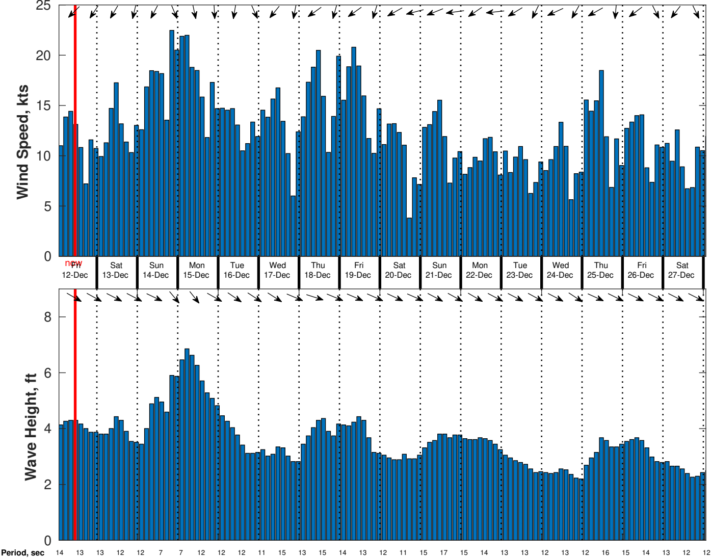
Wind & Wave Forecast for CSA (ONHYM) PPL EBS - Mauritania from 11-Dec-2025 01:00:00 to 27-Dec-2025 01:00:00
