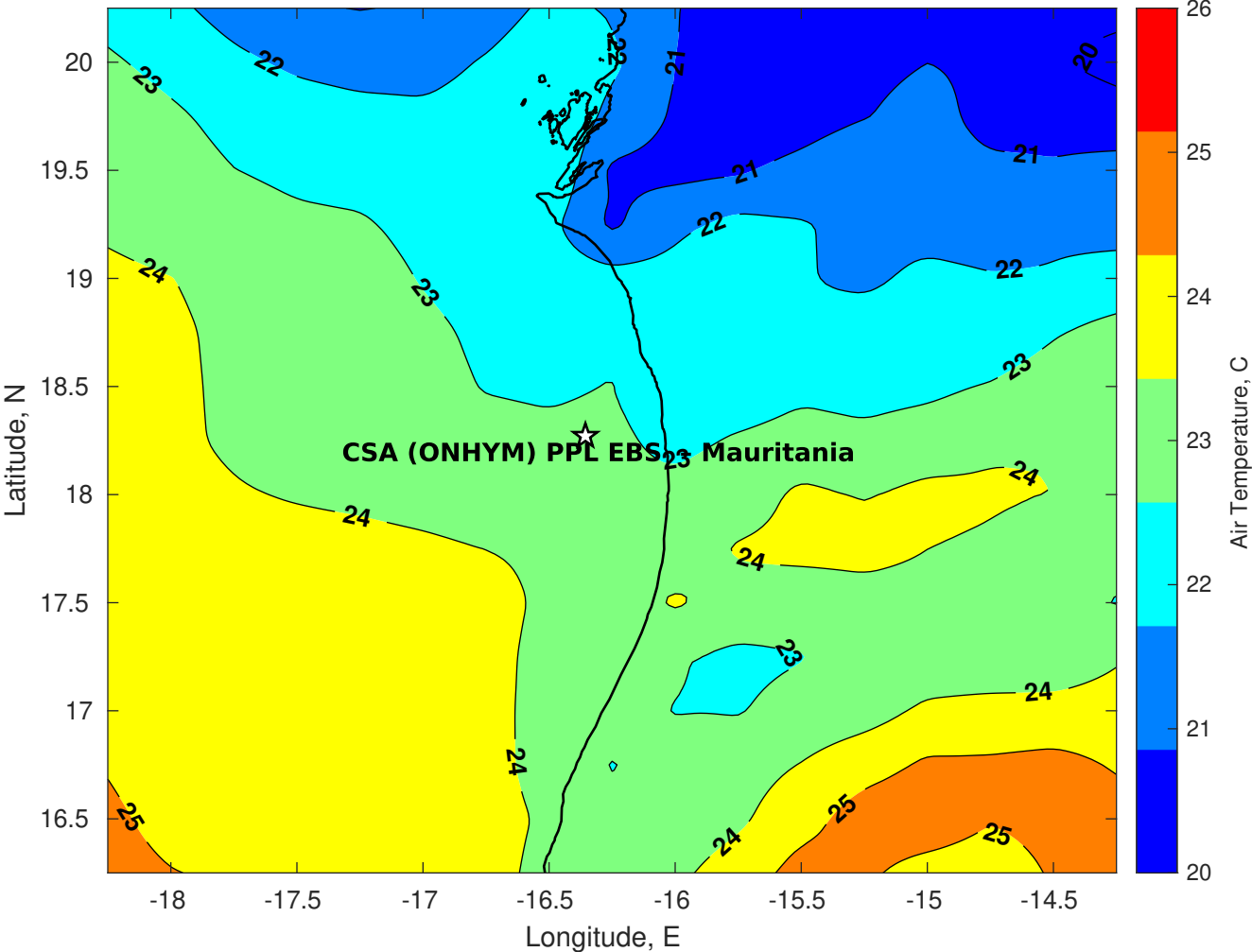
Air Temperature (C) for CSA (ONHYM) PPL EBS - Mauritania at 11-Dec-2025
