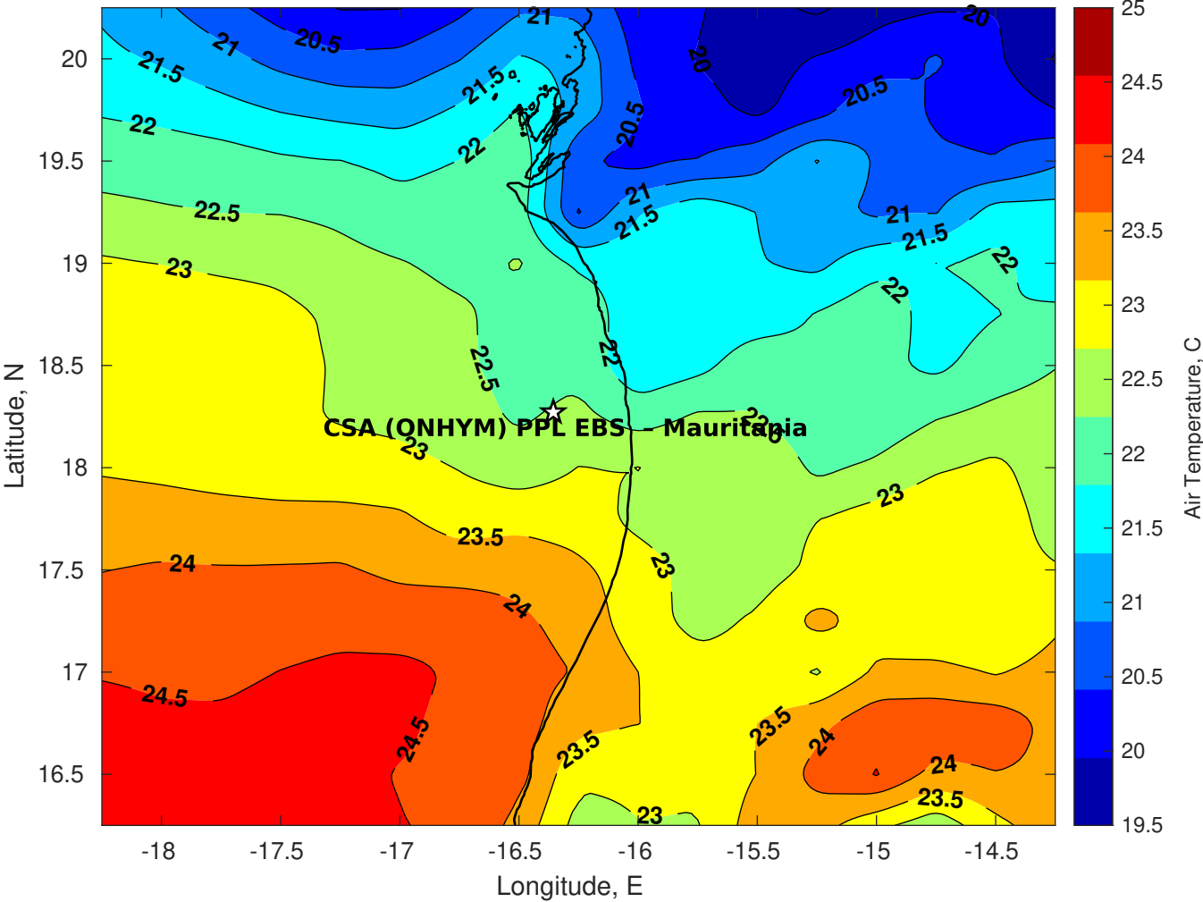
Air Temperature (C) for CSA (ONHYM) PPL EBS - Mauritania at 11-Dec-2025
