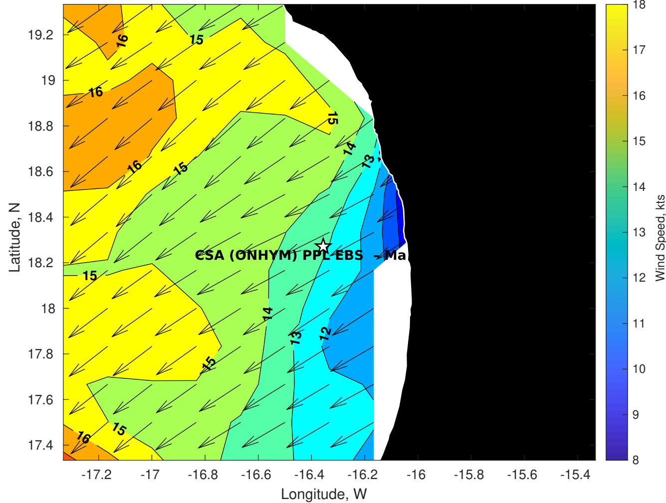
GFS Winds (kts) for CSA (ONHYM) PPL EBS - Mauritania at 11-Dec-2025 09:00:00
