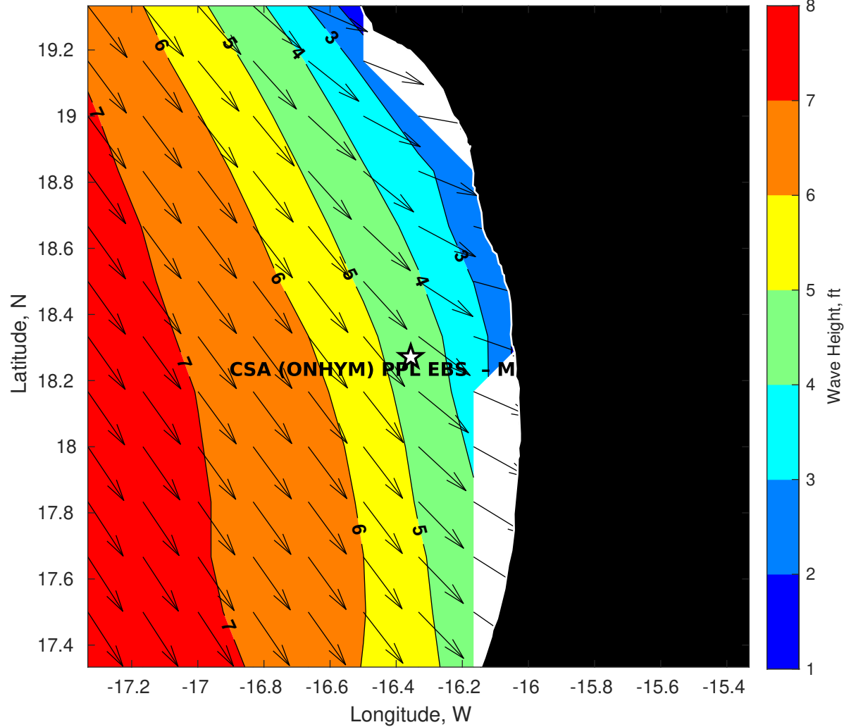
GFS Wave Height (ft) for CSA (ONHYM) PPL EBS - Mauritania at 11-Dec-2025 09:00:00
