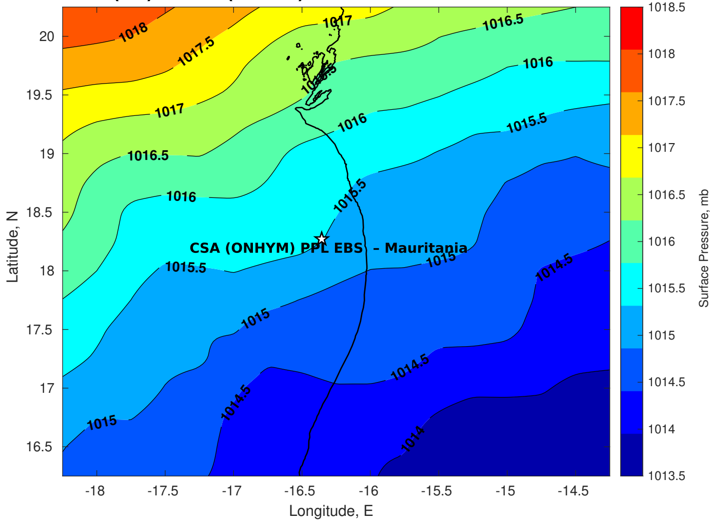
Surface Pressure (mb) for CSA (ONHYM) PPL EBS - Mauritania at 13-Dec-2025 00:00:00
