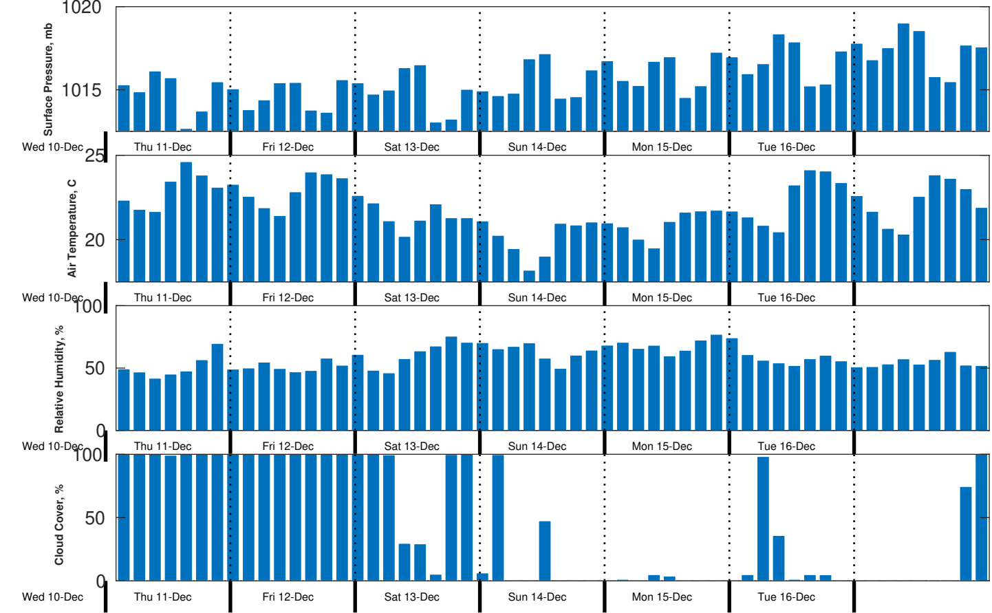
Met Forecast for CSA (ONHYM) PPL EBS - Mauritania from 11-Dec-2025 00:00:00 to 18-Dec-2025 00:00:00
