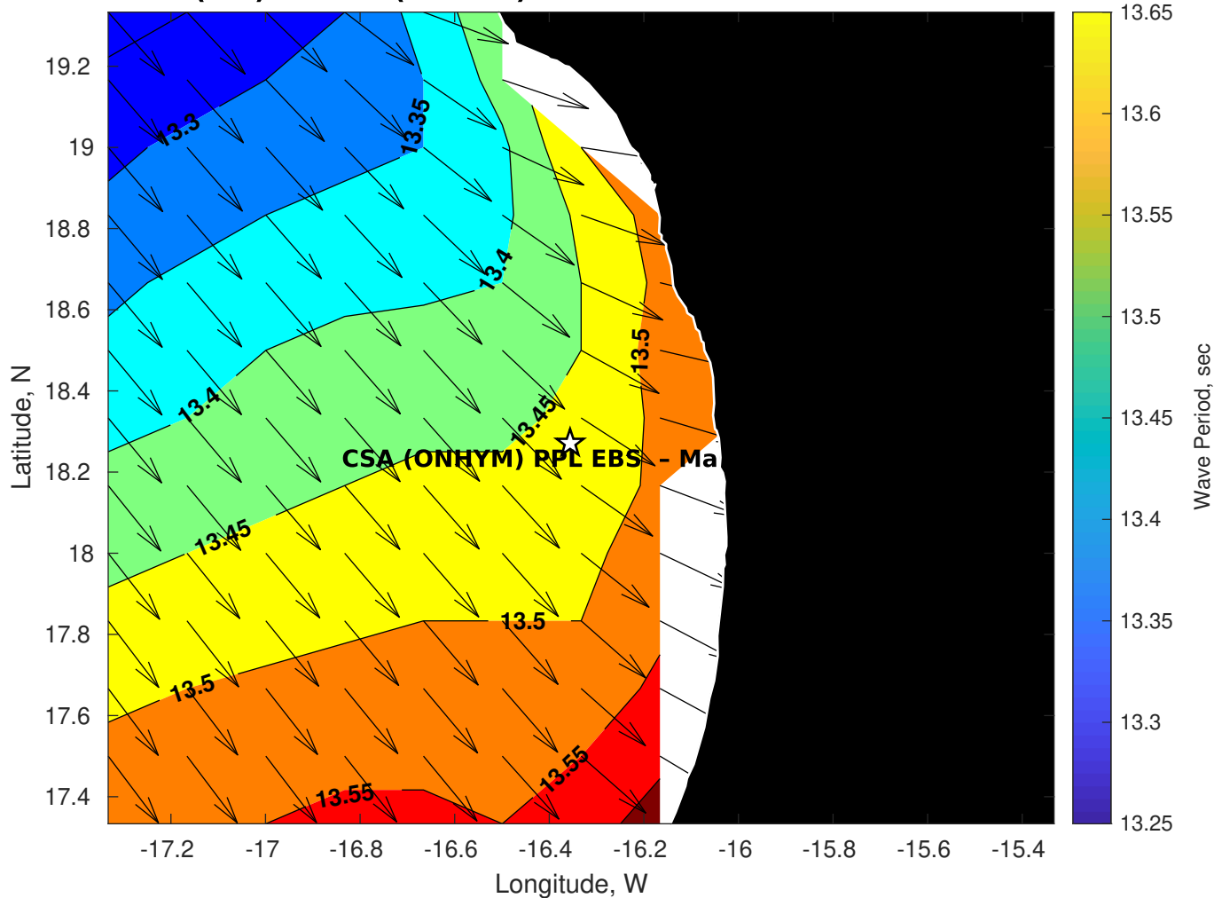
GFS Wave Period (sec) for CSA (ONHYM) PPL EBS - Mauritania at 11-Dec-2025 09:00:00
