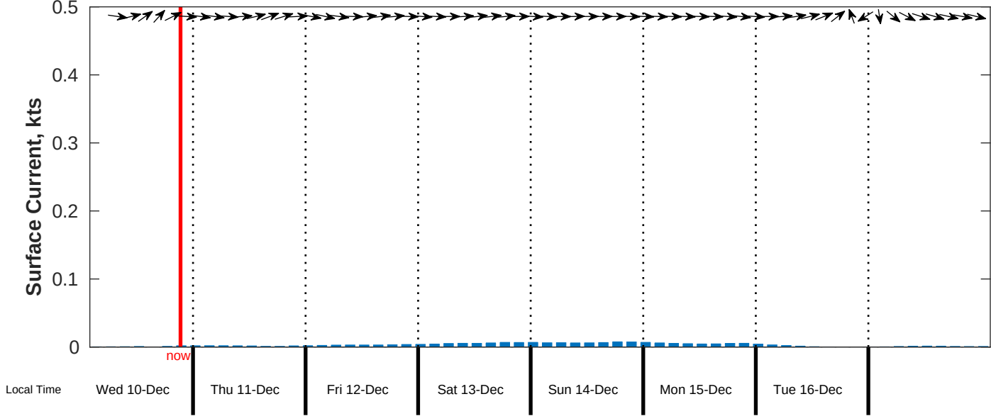
Surface Current Forecast for CSA (ONHYM) PPL EBS - Mauritania from 10-Dec-2025 00:00:00 to 18-Dec-2025 00:00:00
