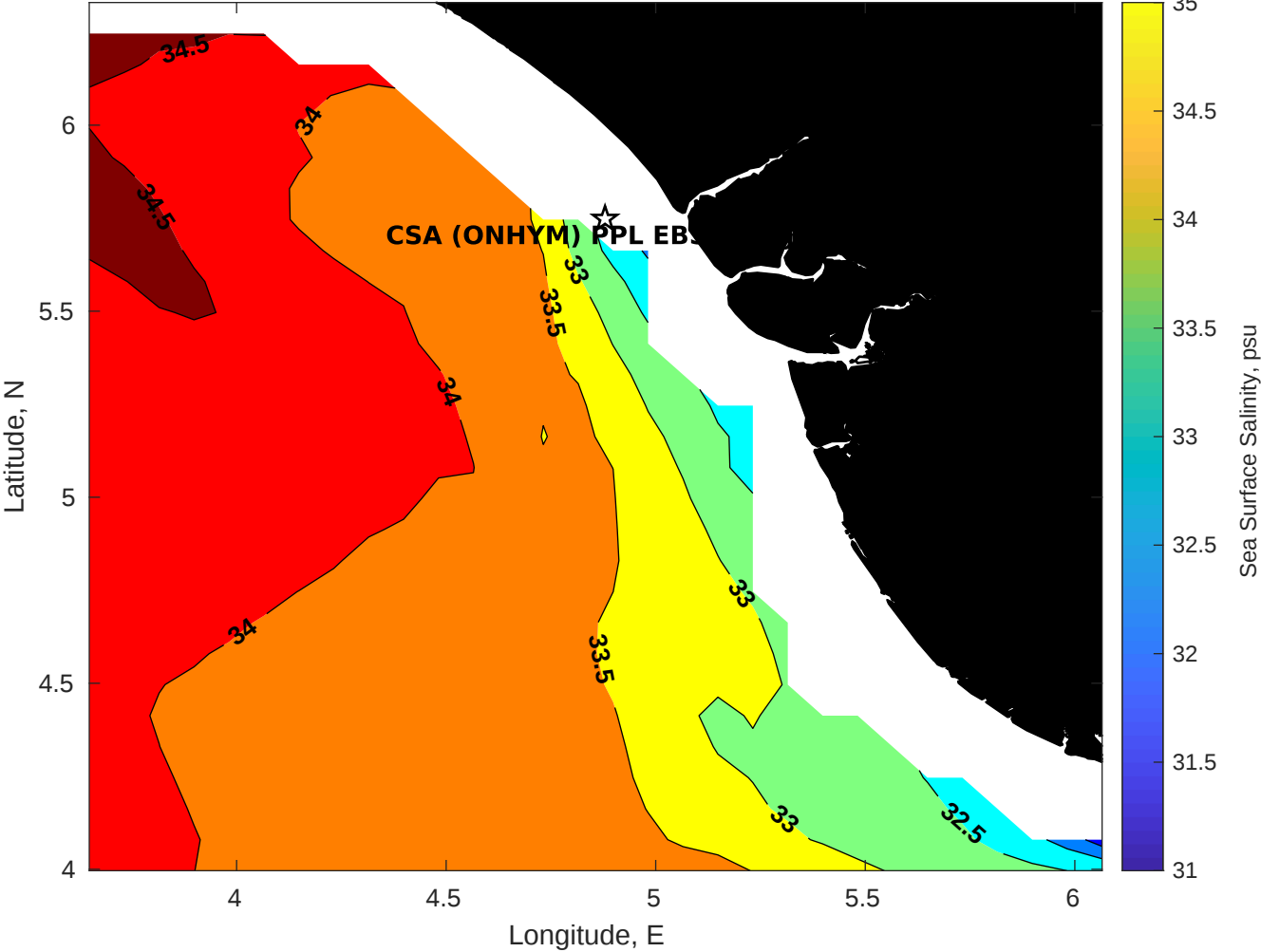
Surface Salinity for CSA (ONHYM) PPL EBS - Nigeria at 10-Dec-2025 00:00:00
