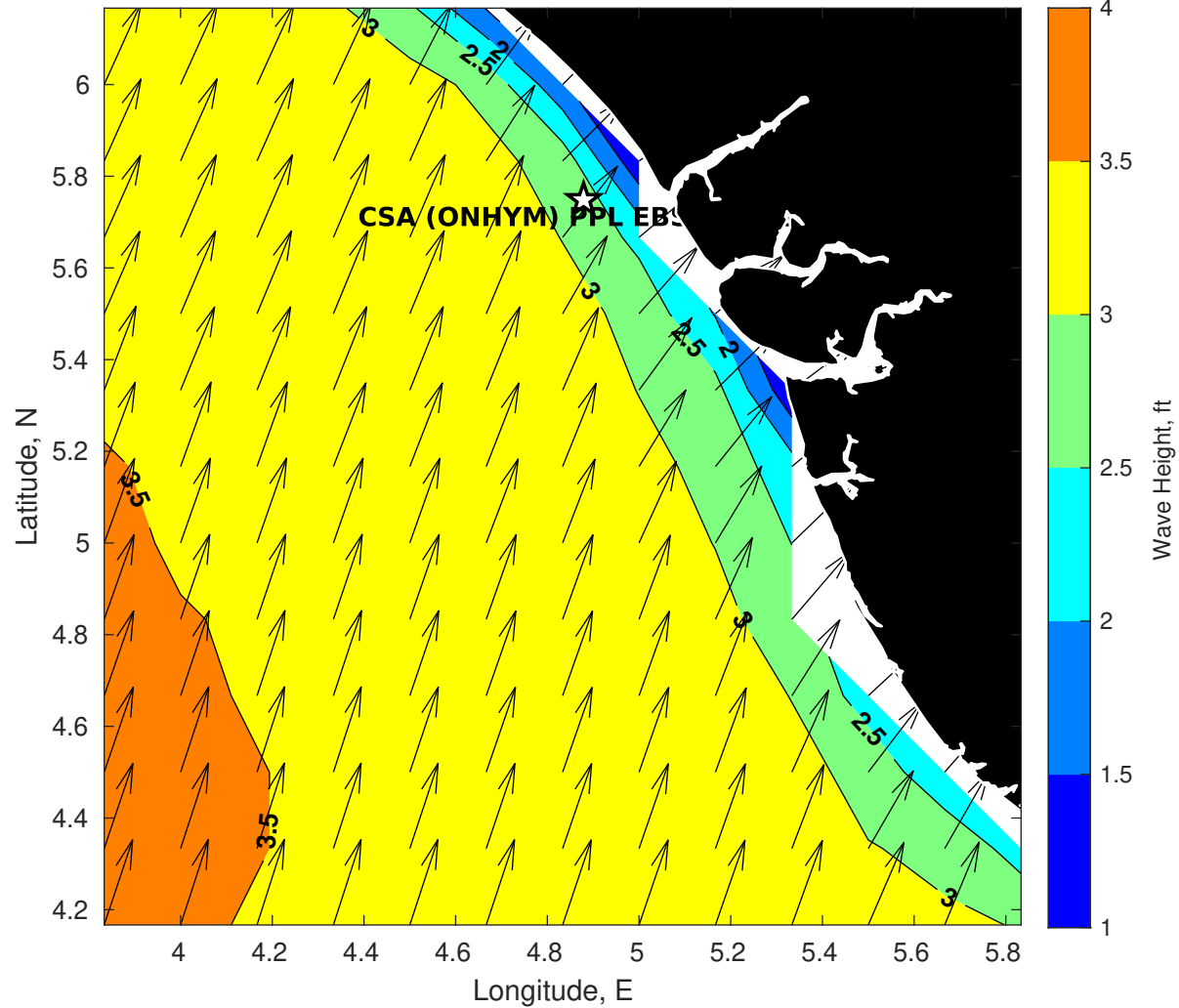
GFS Wave Height (ft) for CSA (ONHYM) PPL EBS - Nigeria at 11-Dec-2025 09:00:00
