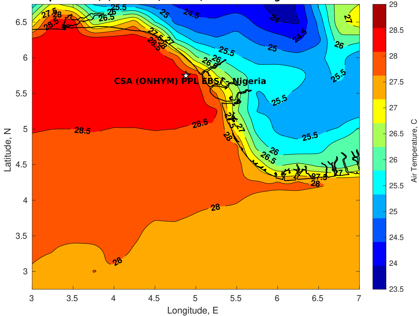
Air Temperature (C) for CSA (ONHYM) PPL EBS - Nigeria at 11-Dec-2025
