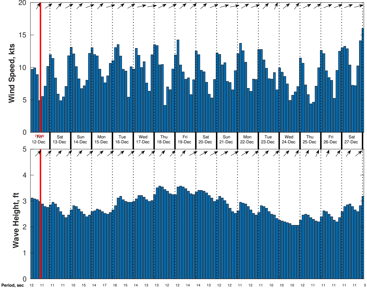
Wind & Wave Forecast for CSA (ONHYM) PPL EBS - Nigeria from 11-Dec-2025 02:00:00 to 27-Dec-2025 02:00:00
