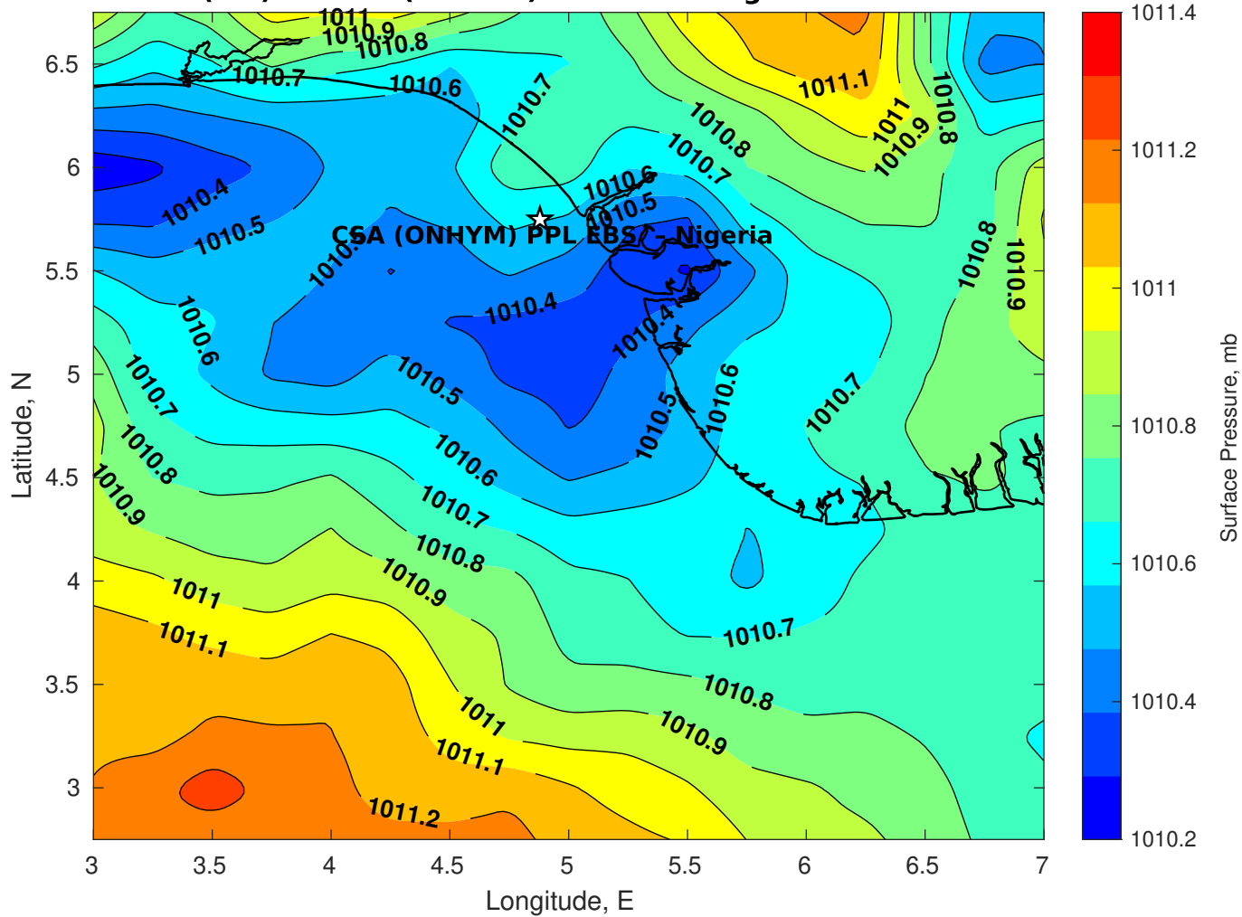
Surface Pressure (mb) for CSA (ONHYM) PPL EBS - Nigeria at 12-Dec-2025 00:00:00
