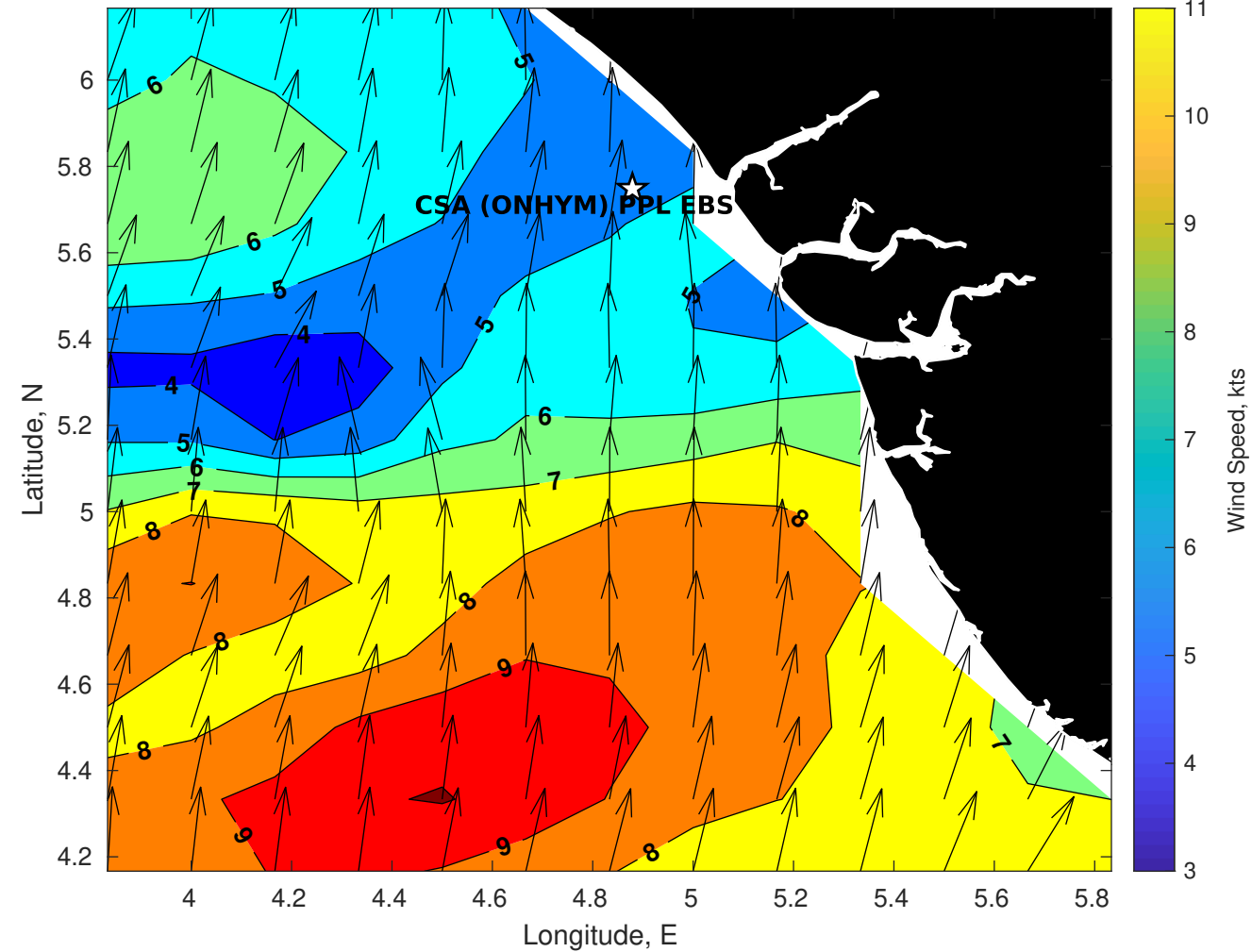
GFS Winds (kts) for CSA (ONHYM) PPL EBS - Nigeria at 11-Dec-2025 09:00:00
