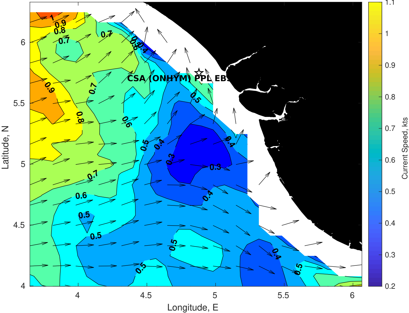
Surface Currents for CSA (ONHYM) PPL EBS - Nigeria at 10-Dec-2025 00:00:00
