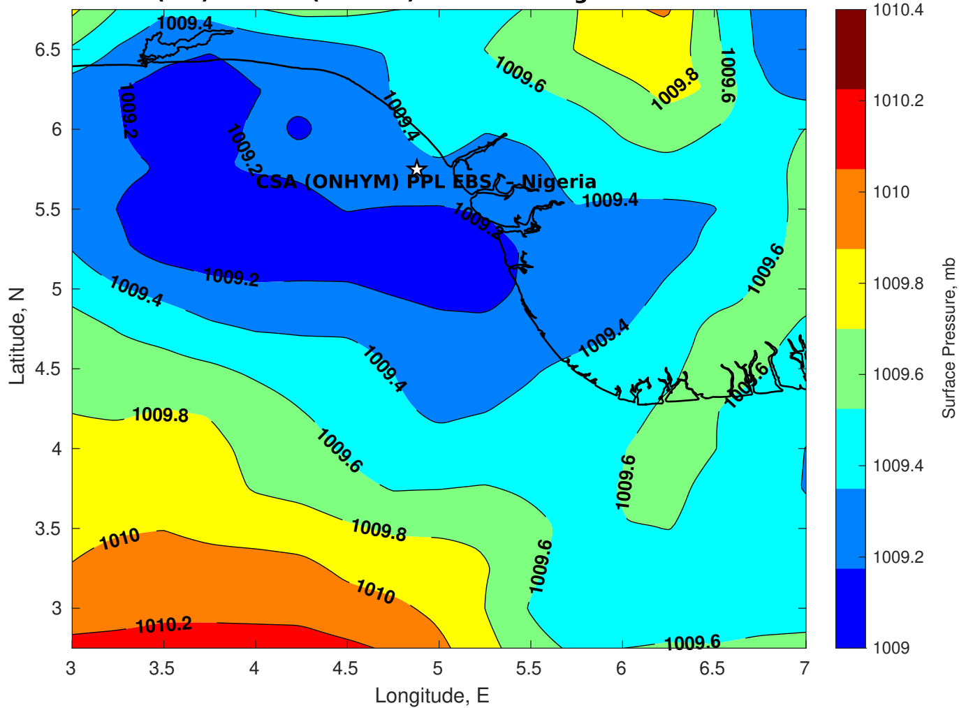
Surface Pressure (mb) for CSA (ONHYM) PPL EBS - Nigeria at 13-Dec-2025 00:00:00
