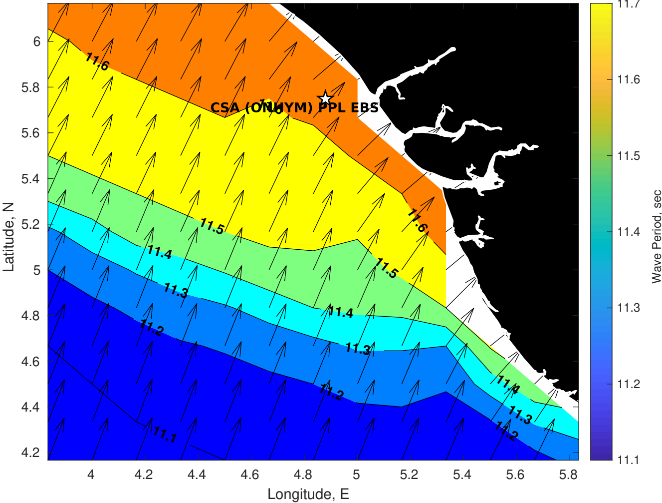
GFS Wave Period (sec) for CSA (ONHYM) PPL EBS - Nigeria at 11-Dec-2025 09:00:00
