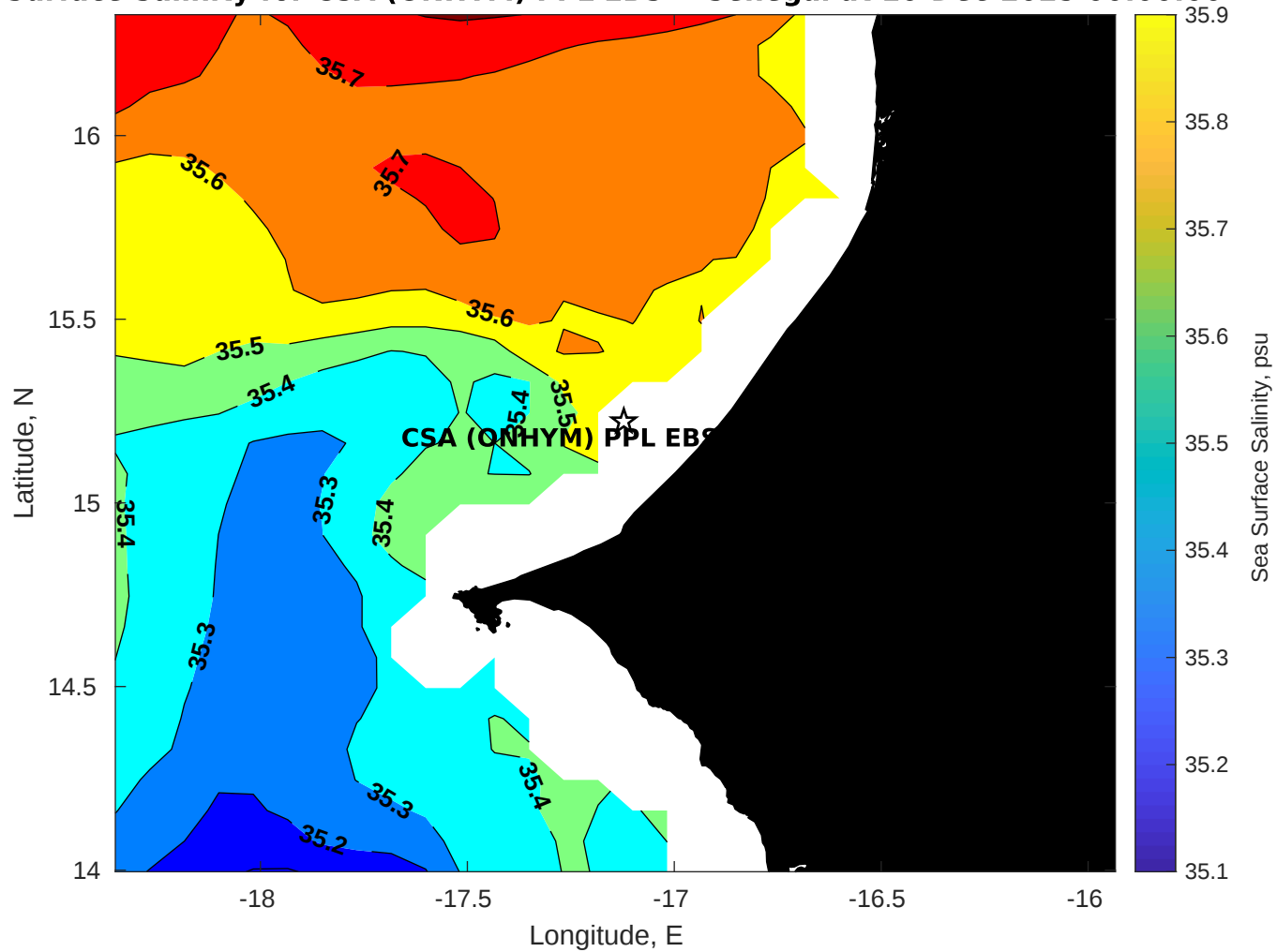
Surface Salinity for CSA (ONHYM) PPL EBS - Senegal at 10-Dec-2025 00:00:00
