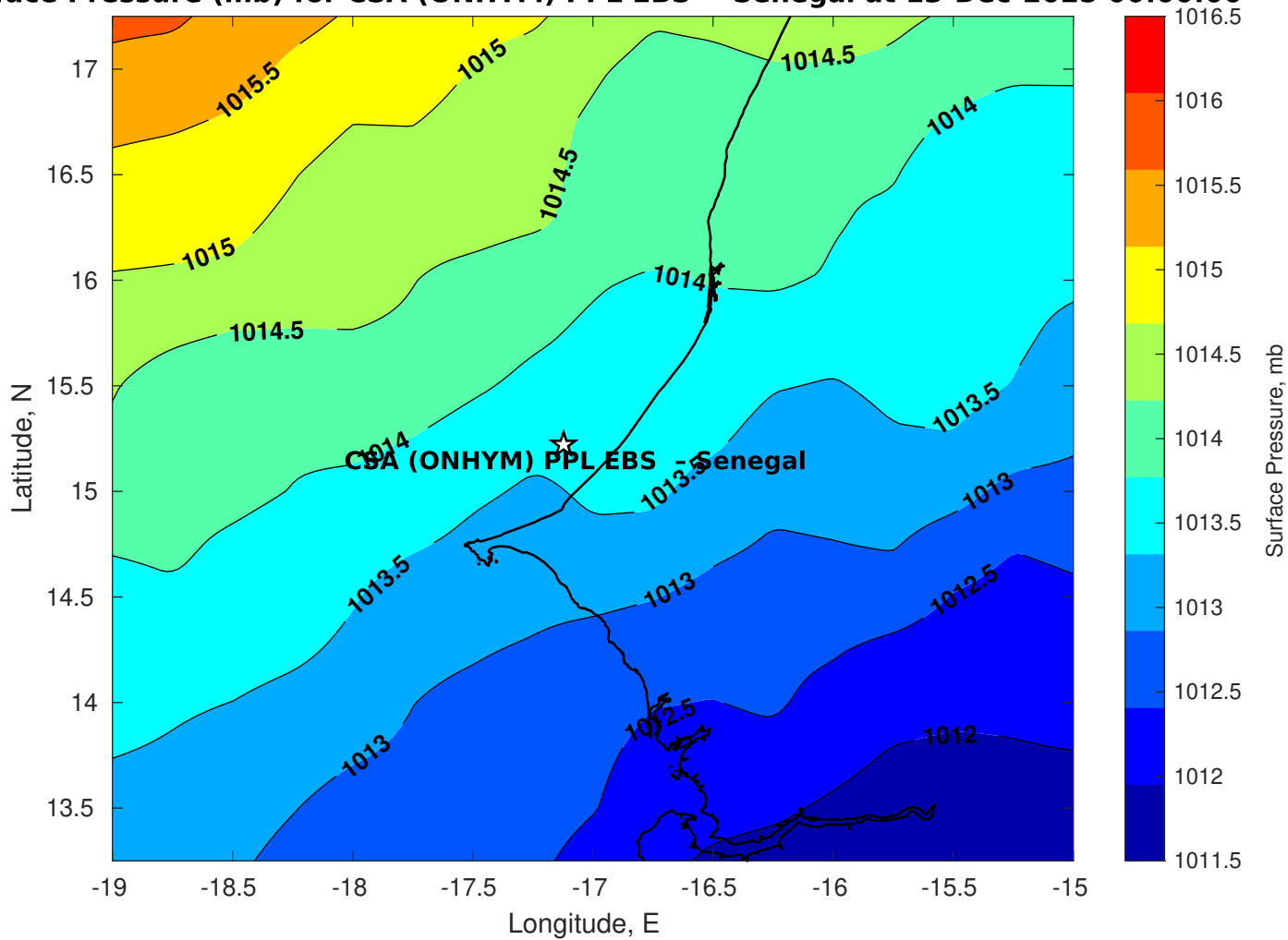
Surface Pressure (mb) for CSA (ONHYM) PPL EBS - Senegal at 13-Dec-2025 00:00:00
