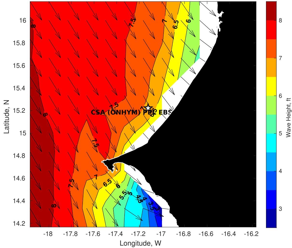
GFS Wave Height (ft) for CSA (ONHYM) PPL EBS - Senegal at 11-Dec-2025 09:00:00
