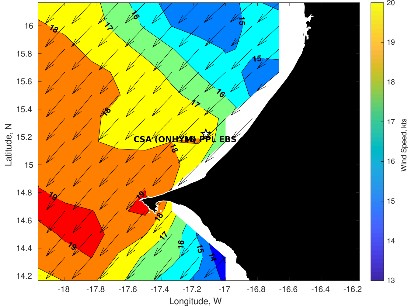
GFS Winds (kts) for CSA (ONHYM) PPL EBS - Senegal at 11-Dec-2025 09:00:00
