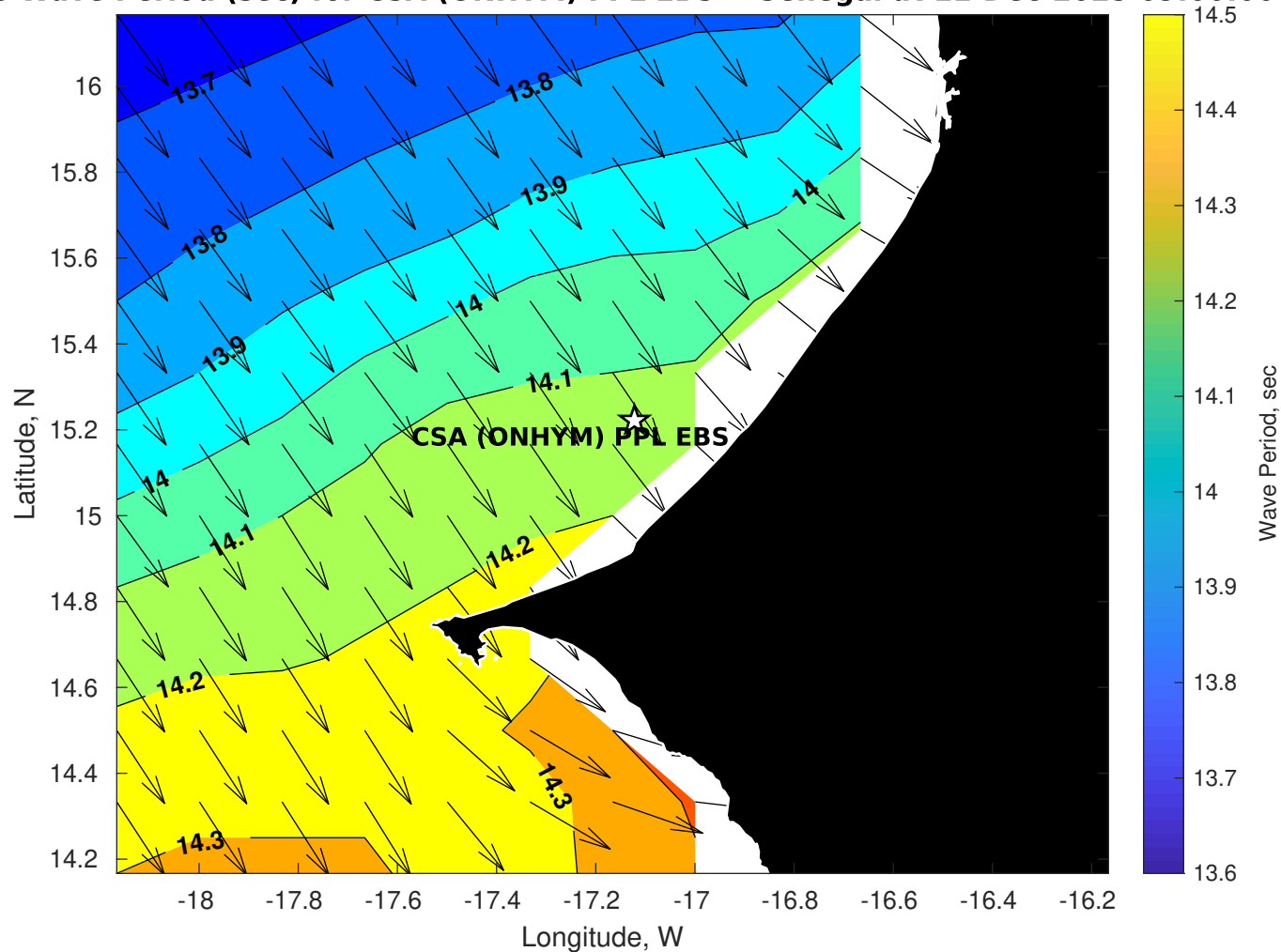
GFS Wave Period (sec) for CSA (ONHYM) PPL EBS - Senegal at 11-Dec-2025 09:00:00
