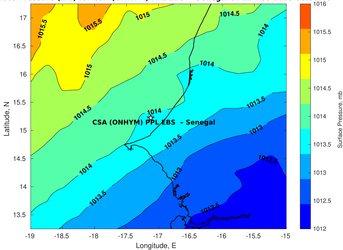
Surface Pressure (mb) for CSA (ONHYM) PPL EBS - Senegal at 12-Dec-2025 00:00:00
