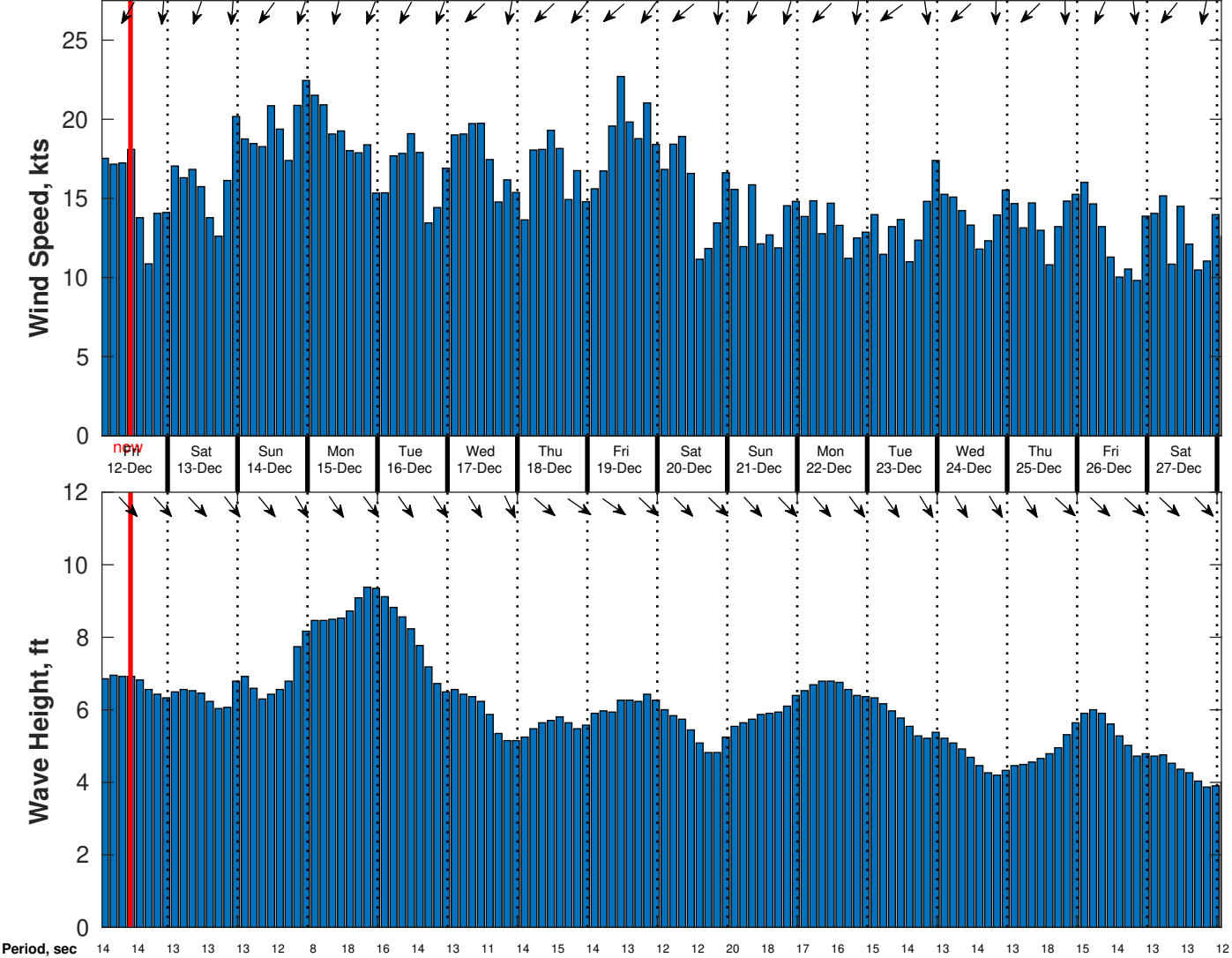
Wind & Wave Forecast for CSA (ONHYM) PPL EBS - Senegal from 11-Dec-2025 01:00:00 to 27-Dec-2025 01:00:00
