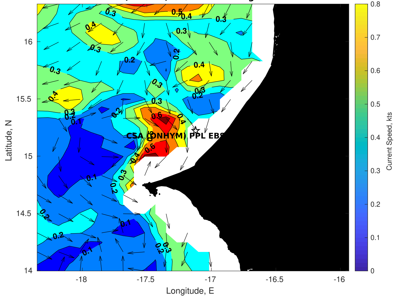
Surface Currents for CSA (ONHYM) PPL EBS - Senegal at 10-Dec-2025 00:00:00
