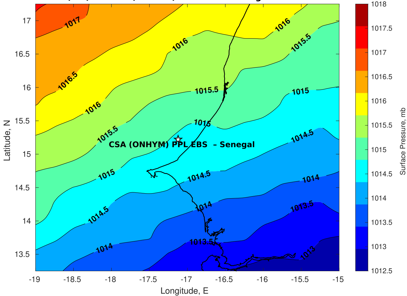
Surface Pressure (mb) for CSA (ONHYM) PPL EBS - Senegal at 11-Dec-2025 00:00:00
