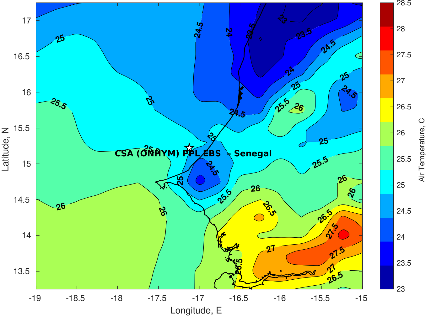
Air Temperature (C) for CSA (ONHYM) PPL EBS - Senegal at 11-Dec-2025
