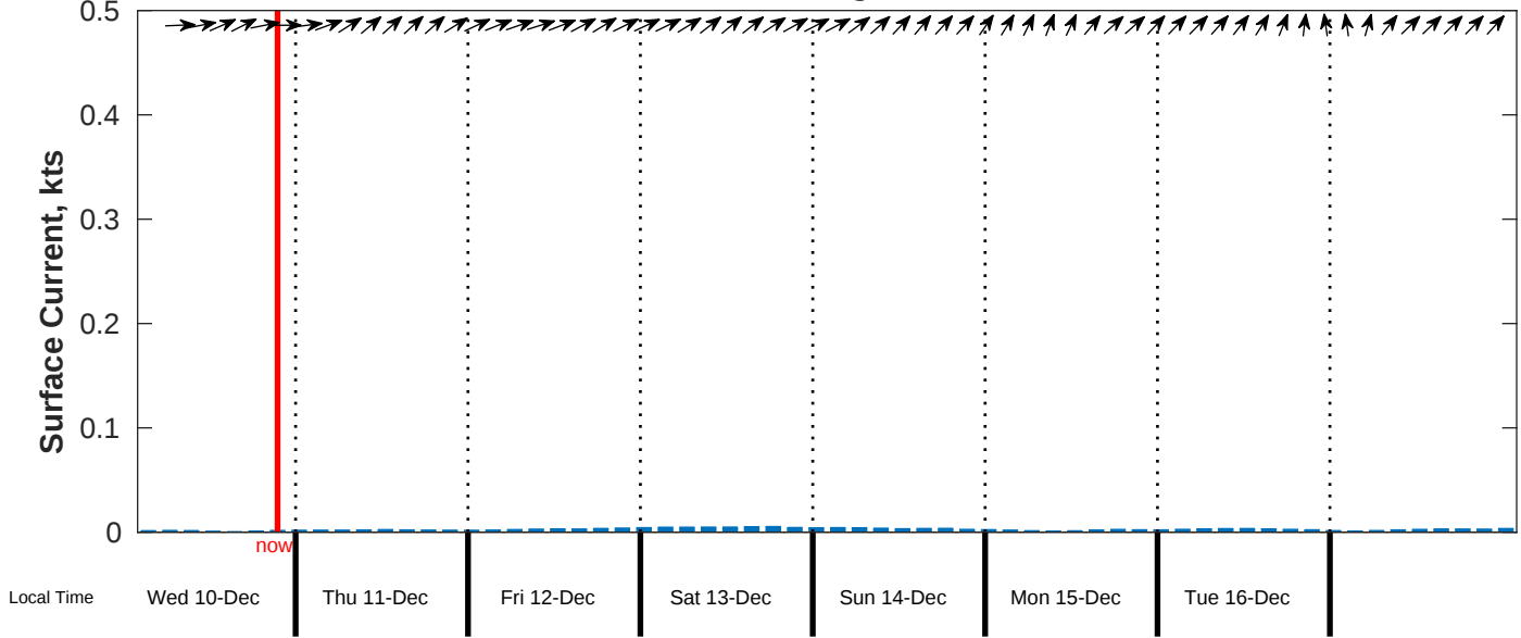
Surface Current Forecast for CSA (ONHYM) PPL EBS - Senegal from 10-Dec-2025 00:00:00 to 18-Dec-2025 00:00:00
