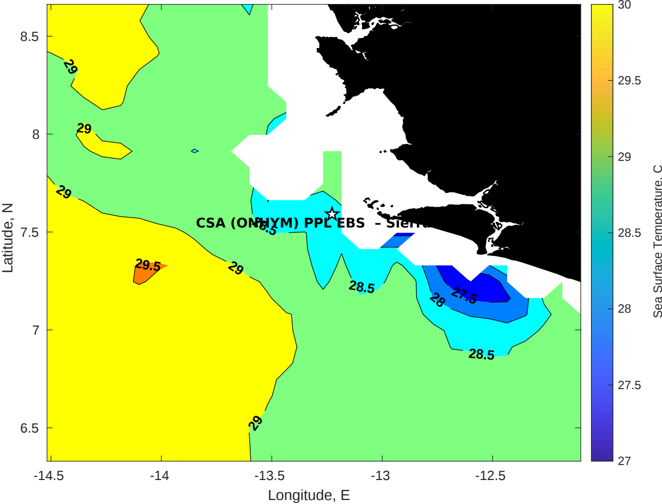
SST for CSA (ONHYM) PPL EBS - Sierra Leone at 10-Dec-2025 00:00:00
