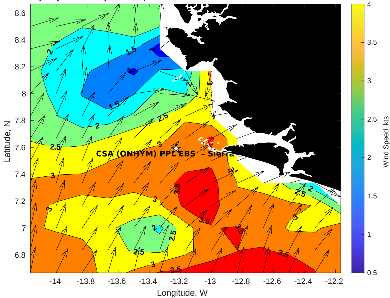
GFS Winds (kts) for CSA (ONHYM) PPL EBS - Sierra Leone at 11-Dec-2025 09:00:00
