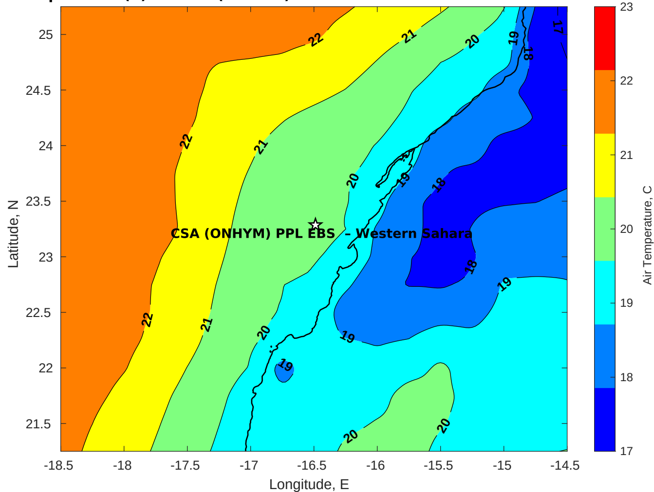
Air Temperature (C) for CSA (ONHYM) PPL EBS - Western Sahara at 11-Dec-2025
