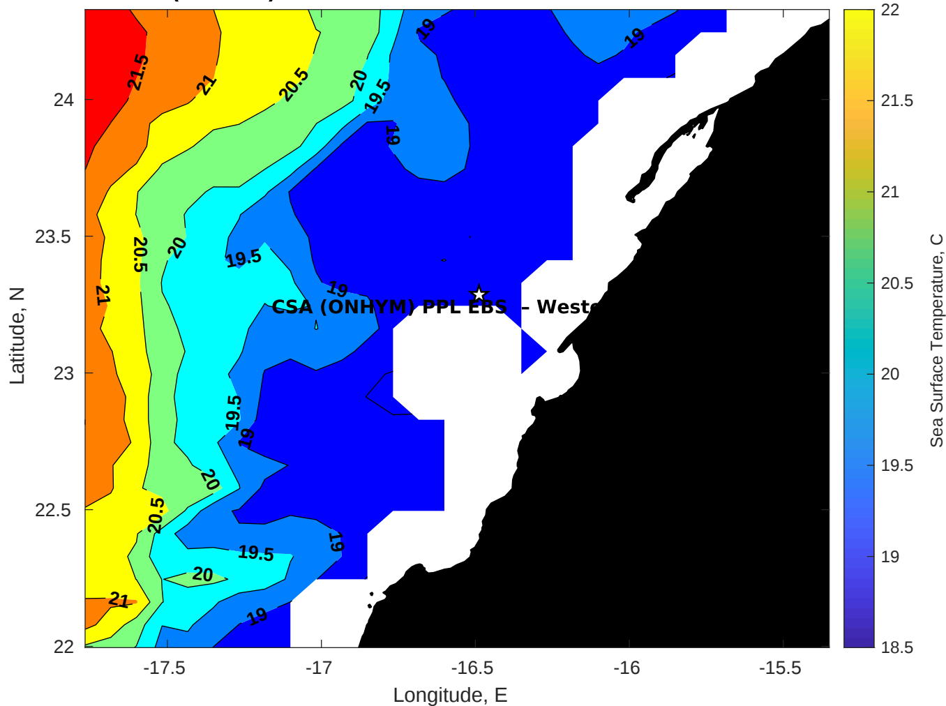
SST for CSA (ONHYM) PPL EBS - Western Sahara at 10-Dec-2025 00:00:00
