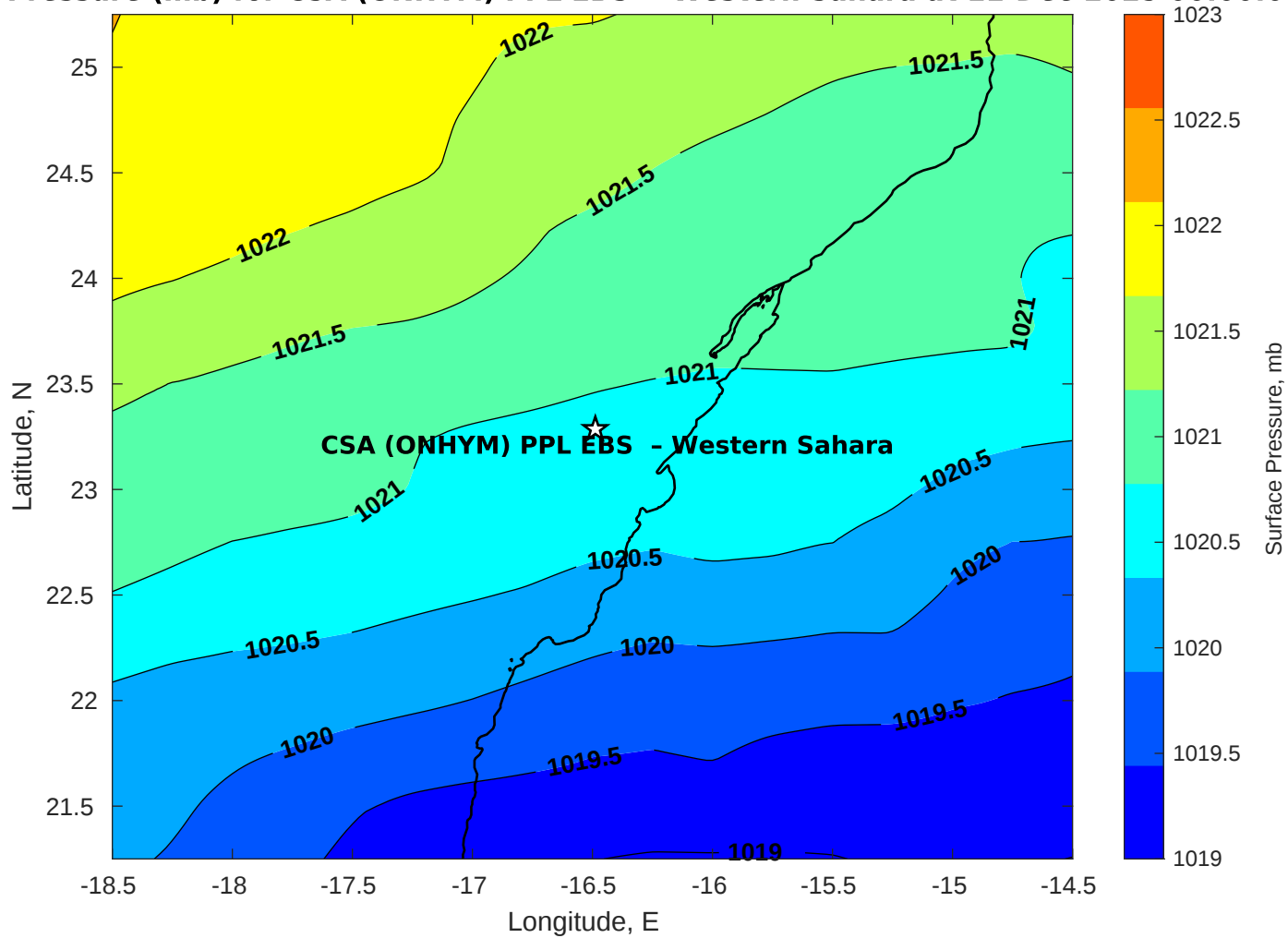
Surface Pressure (mb) for CSA (ONHYM) PPL EBS - Western Sahara at 11-Dec-2025 00:00:00
