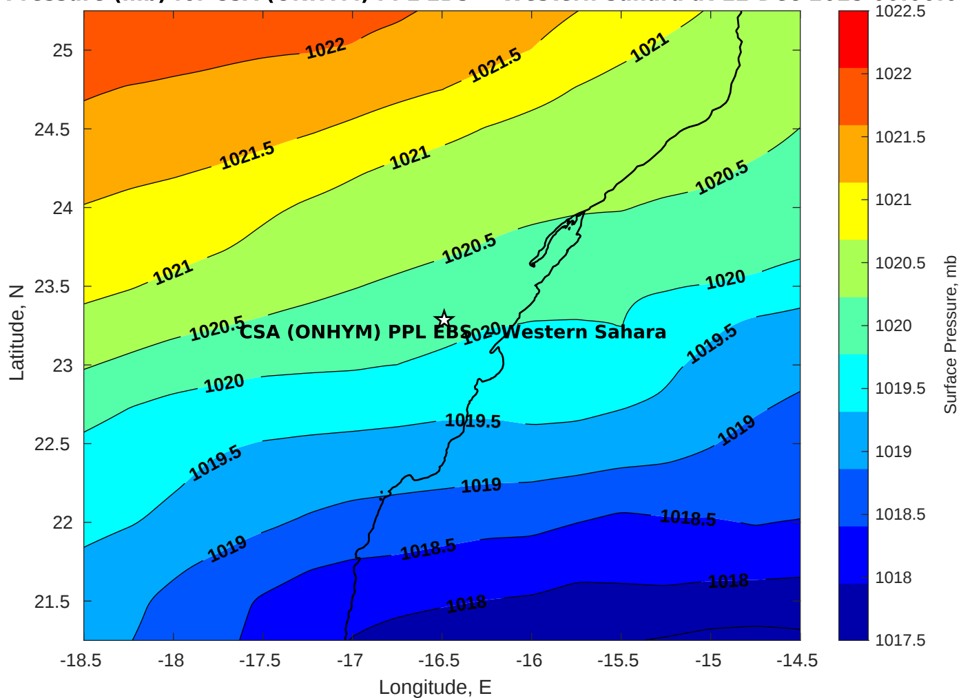
Surface Pressure (mb) for CSA (ONHYM) PPL EBS - Western Sahara at 12-Dec-2025 00:00:00
