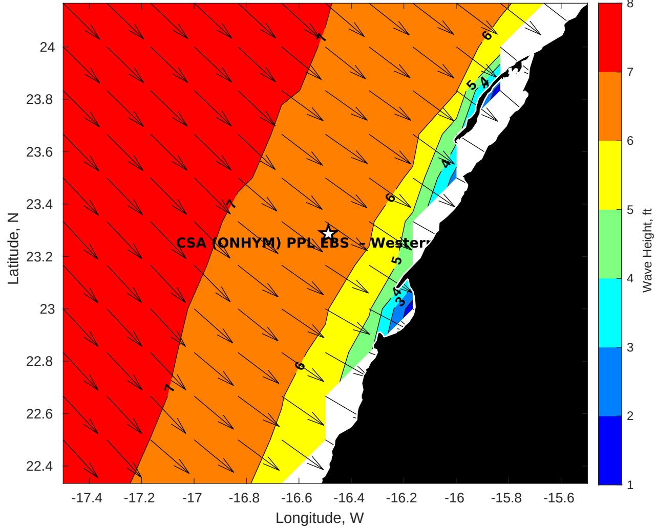
GFS Wave Height (ft) for CSA (ONHYM) PPL EBS - Western Sahara at 11-Dec-2025 09:00:00
