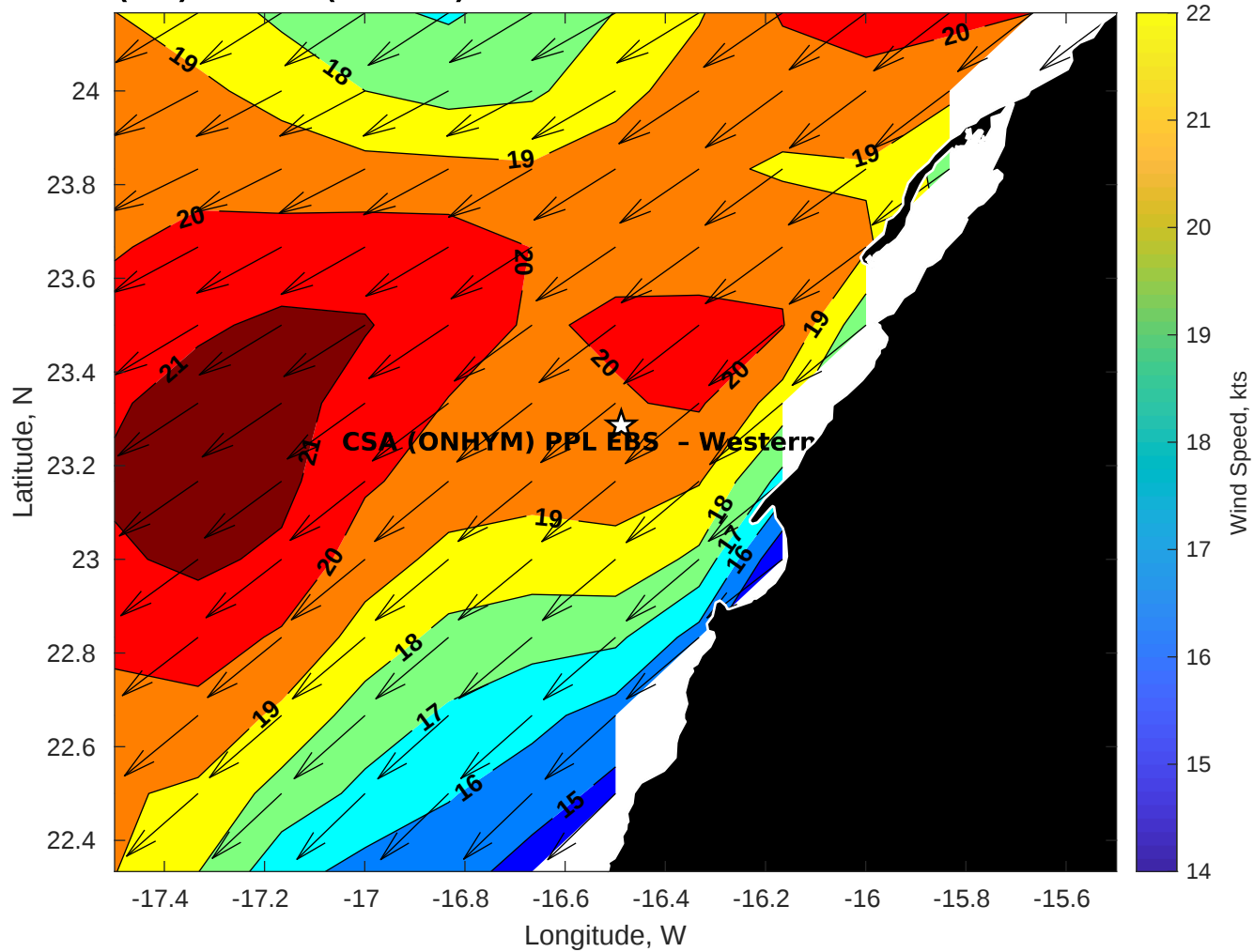
GFS Winds (kts) for CSA (ONHYM) PPL EBS - Western Sahara at 11-Dec-2025 09:00:00
