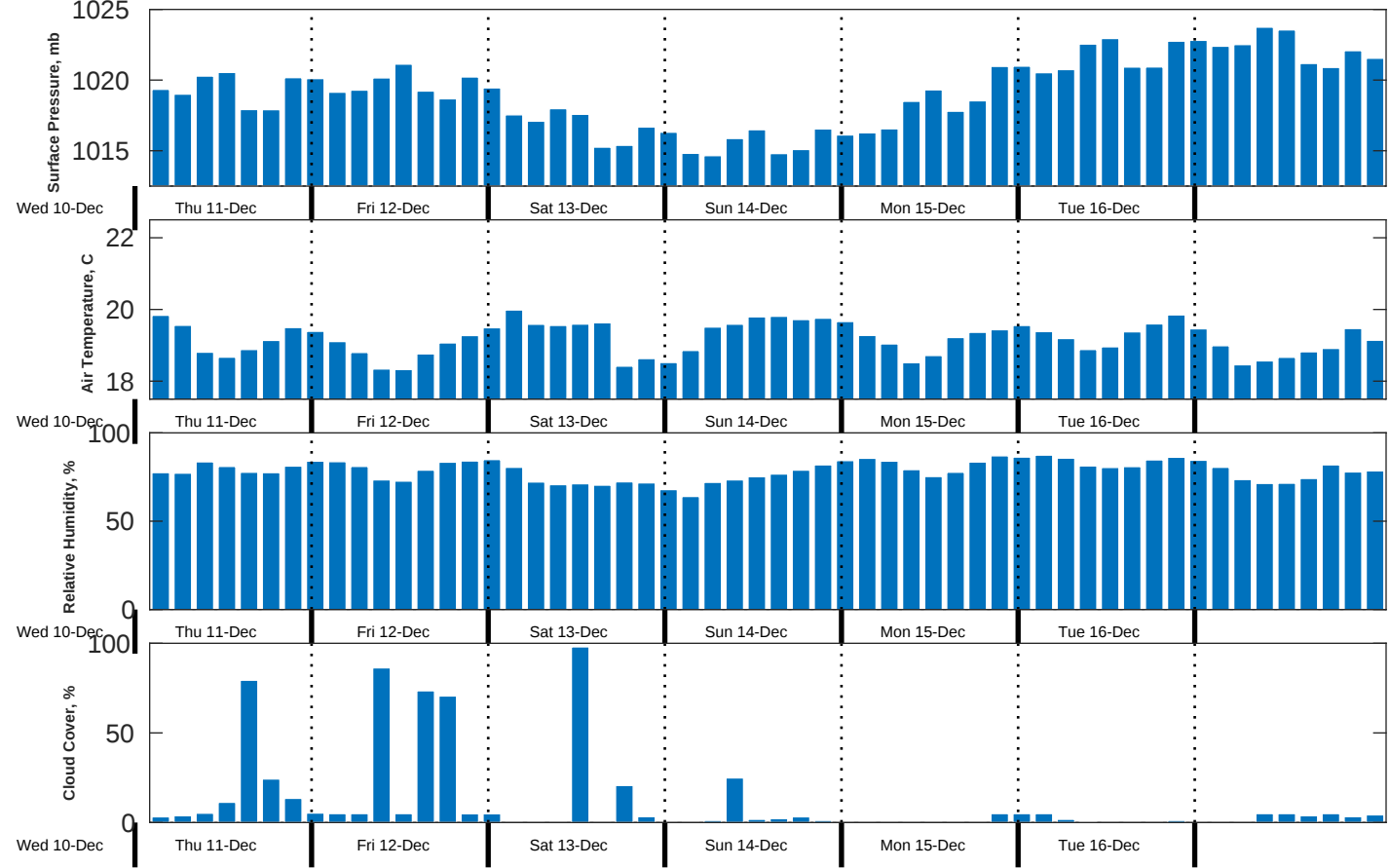
Met Forecast for CSA (ONHYM) PPL EBS - Western Sahara from 11-Dec-2025 00:00:00 to 18-Dec-2025 00:00:00
