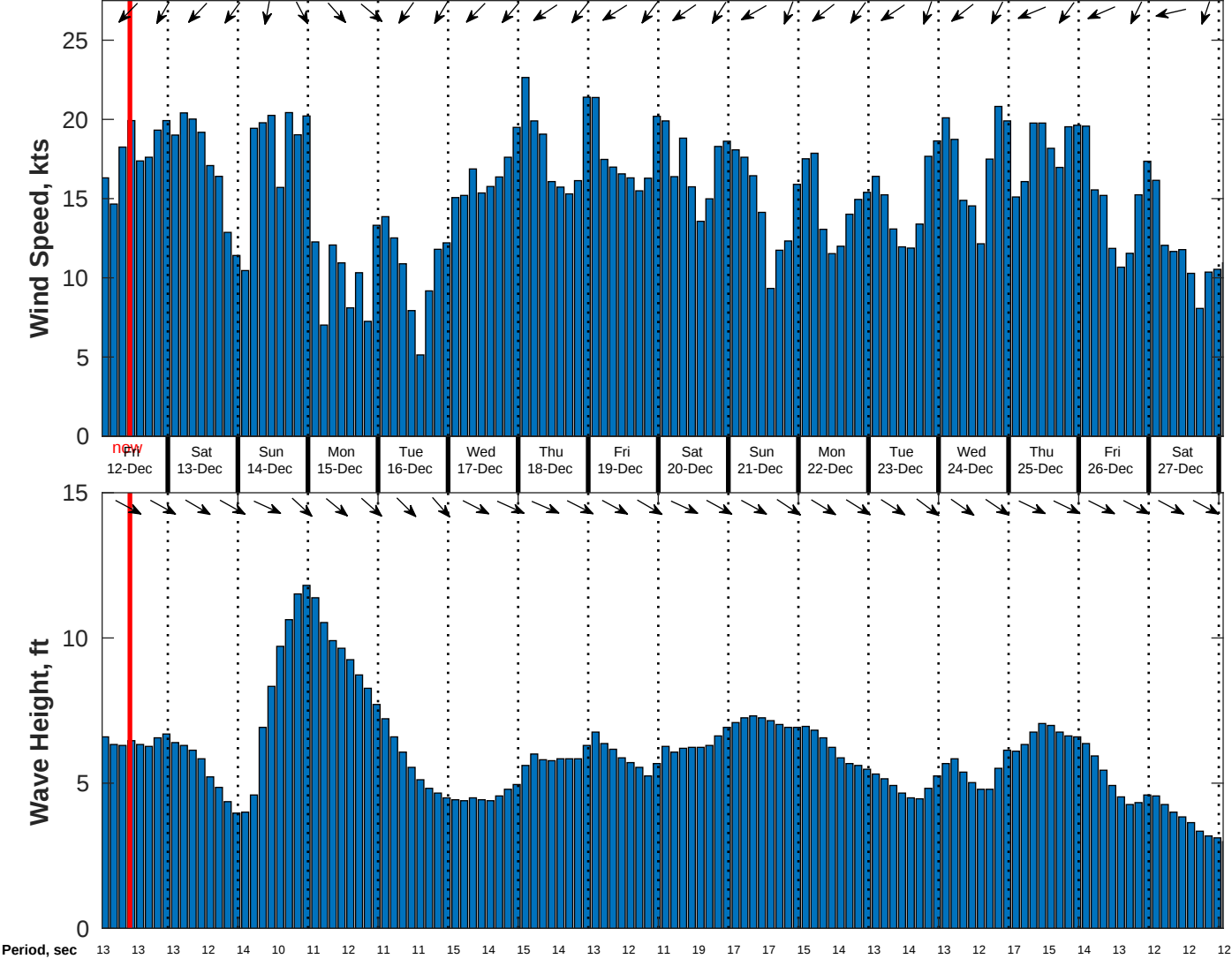
Wind & Wave Forecast for CSA (ONHYM) PPL EBS - Western Sahara from 11-Dec-2025 01:00:00 to 27-Dec-2025 01:00:00
