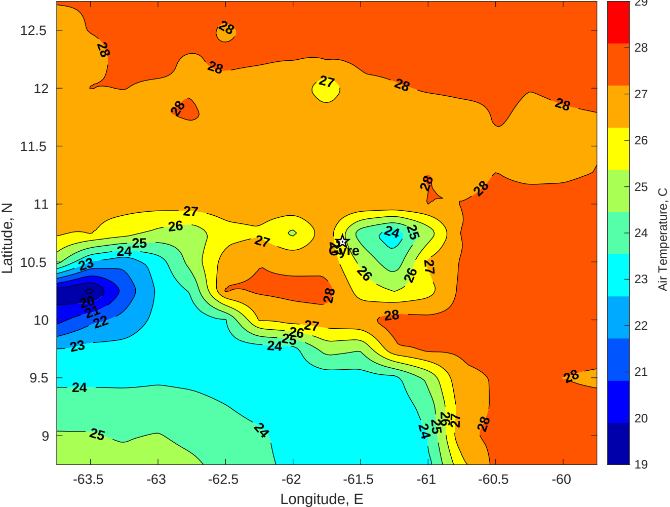
Air Temperature (C) for Gyre at 11-Dec-2025
