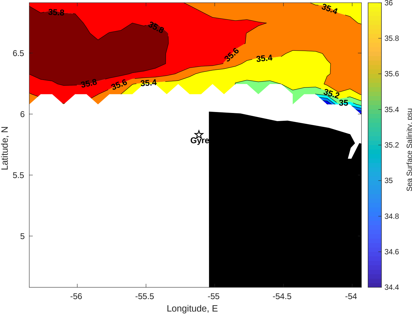
Surface Salinity for Gyre at 10-Dec-2025 00:00:00
