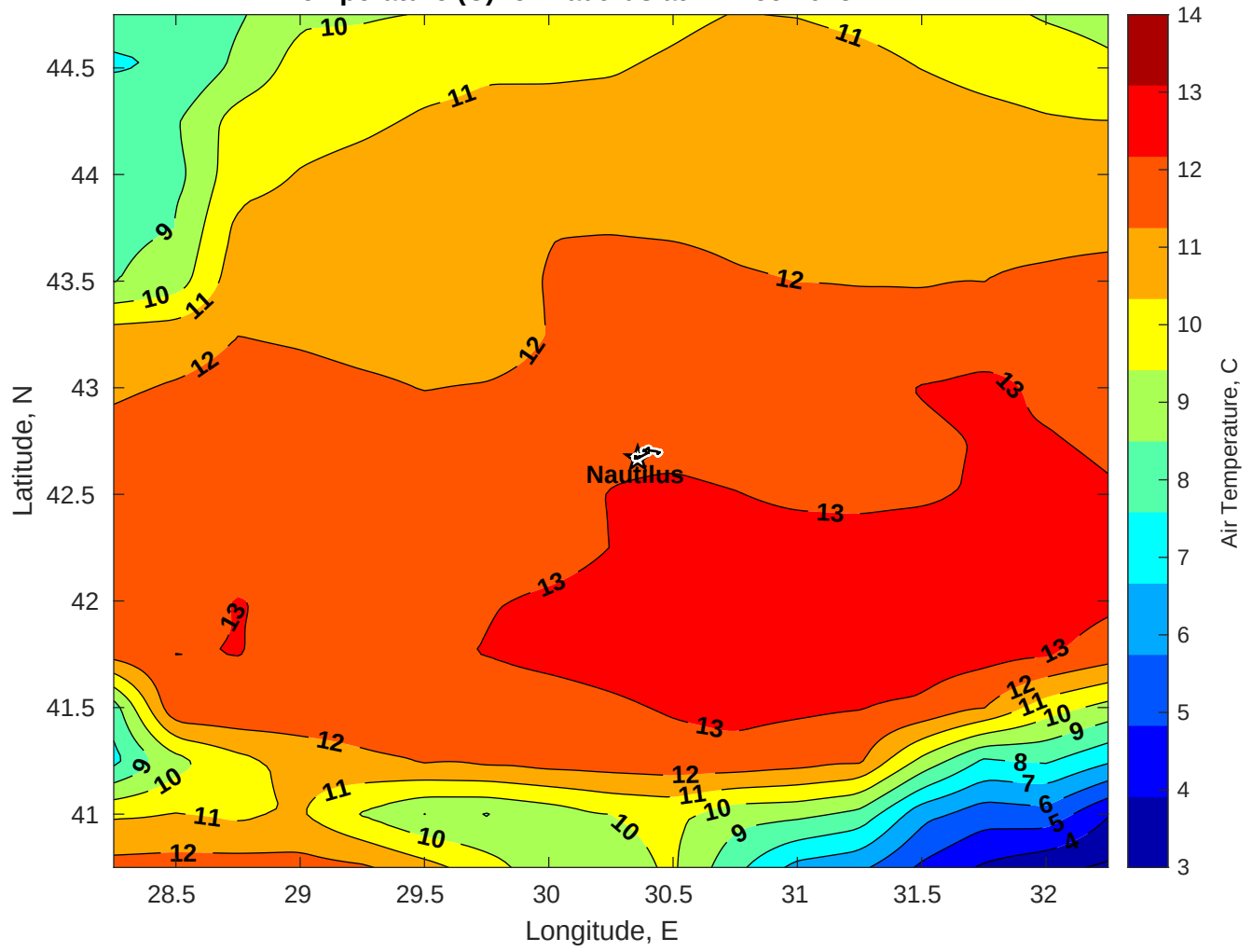
Air Temperature (C) for Nautilus at 11-Dec-2025
