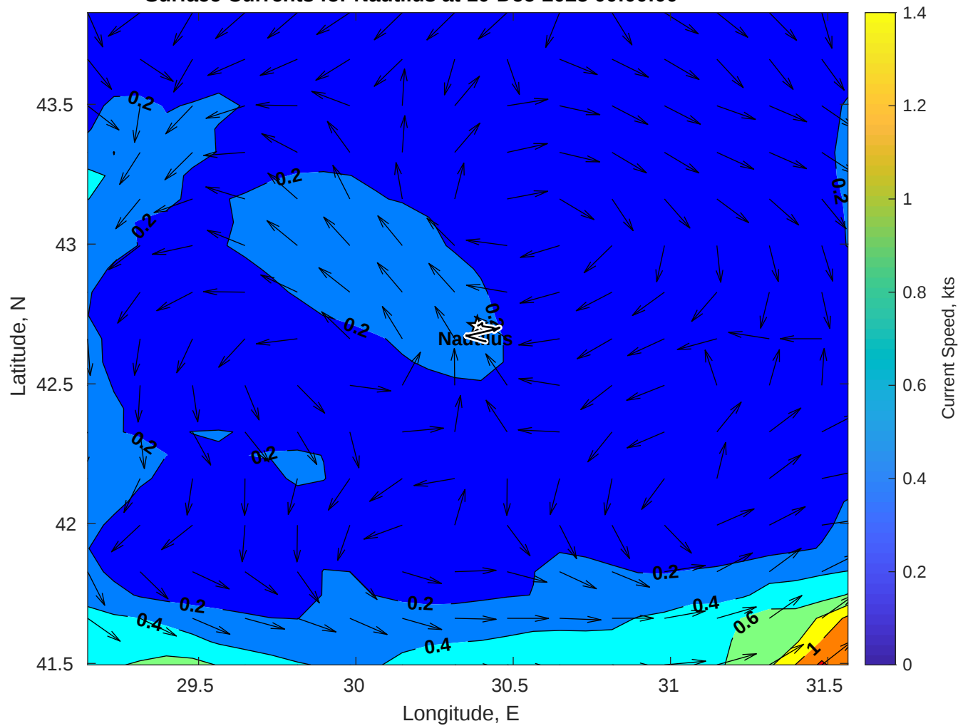
Surface Currents for Nautilus at 10-Dec-2025 00:00:00
