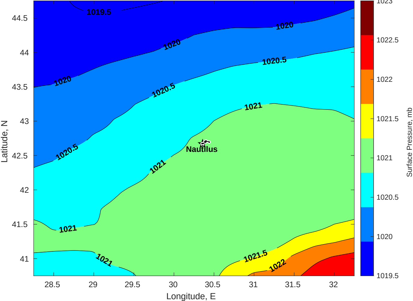
Surface Pressure (mb) for Nautilus at 12-Dec-2025 00:00:00
