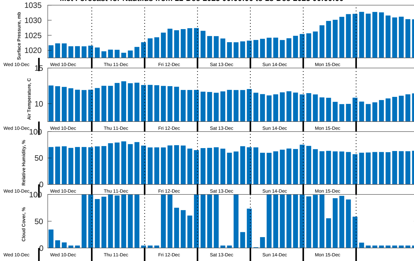
Met Forecast for Nautilus from 11-Dec-2025 00:00:00 to 18-Dec-2025 00:00:00
