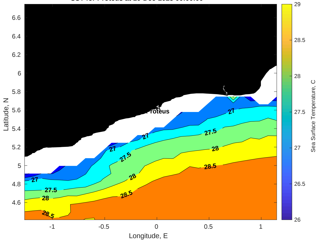
SST for Proteus at 10-Dec-2025 00:00:00
