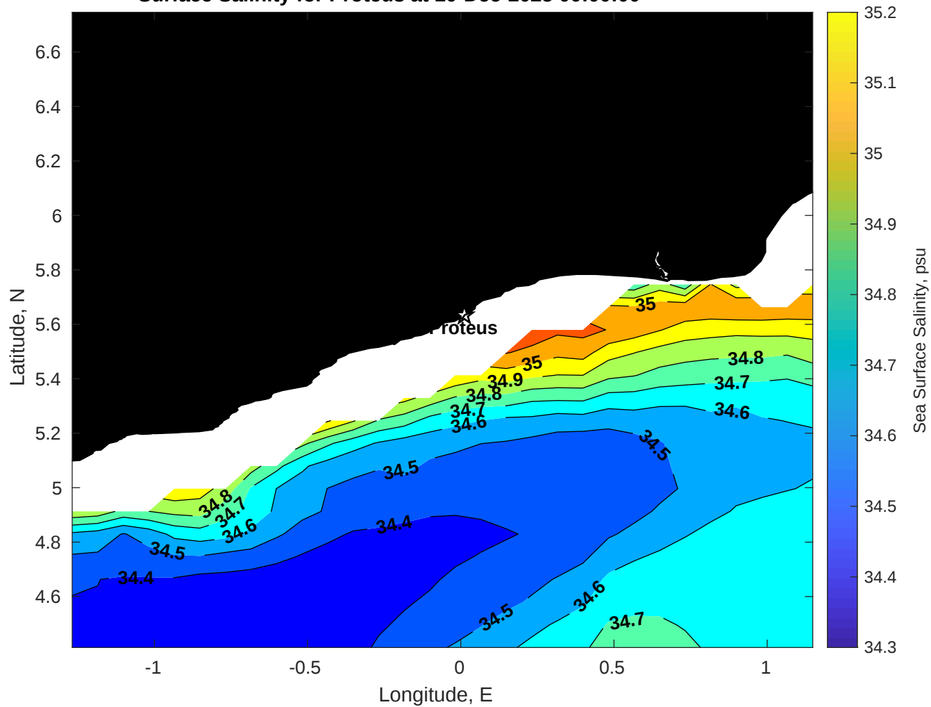
Surface Salinity for Proteus at 10-Dec-2025 00:00:00
