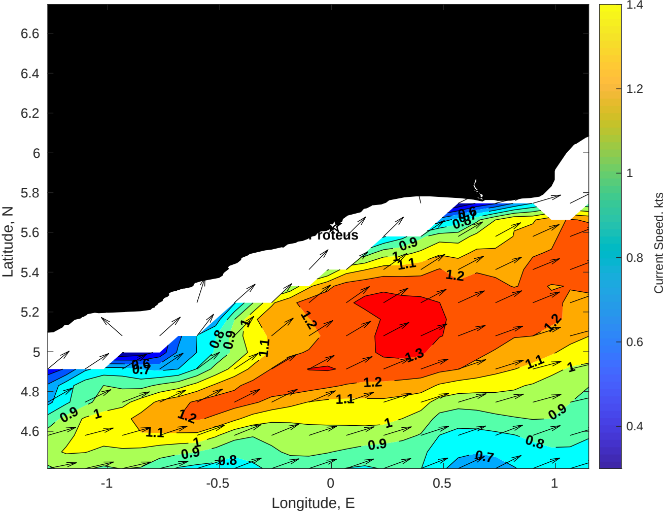
Surface Currents for Proteus at 10-Dec-2025 00:00:00
