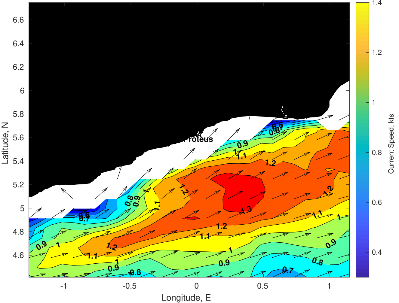
Surface Currents for Proteus at 10-Dec-2025 00:00:00
