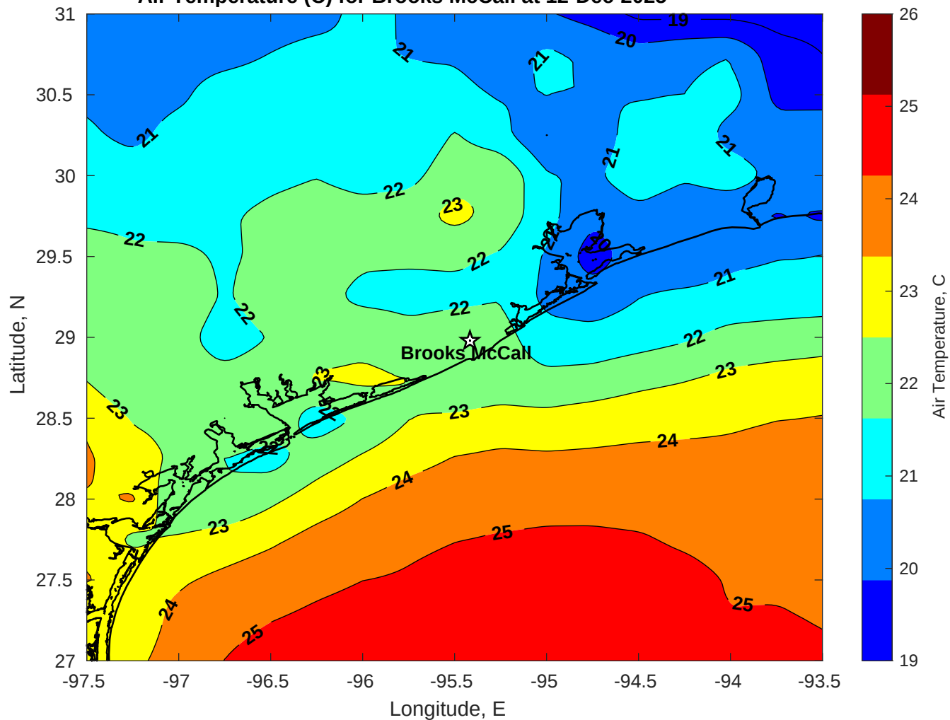
Air Temperature (C) for Brooks McCall at 12-Dec-2025
