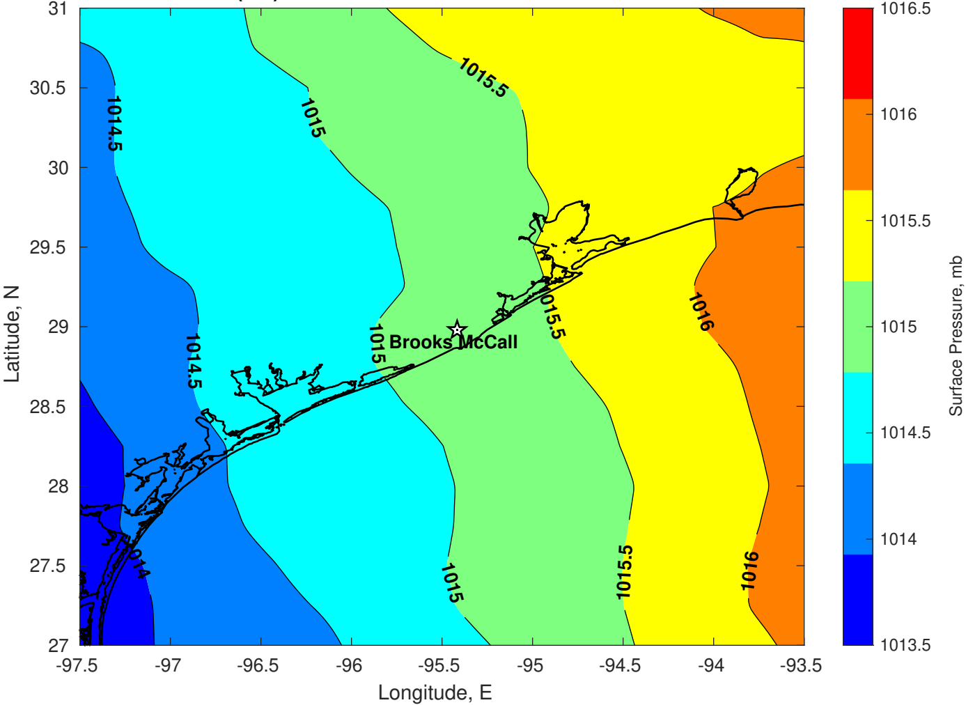
Surface Pressure (mb) for Brooks McCall at 13-Dec-2025 00:00:00
