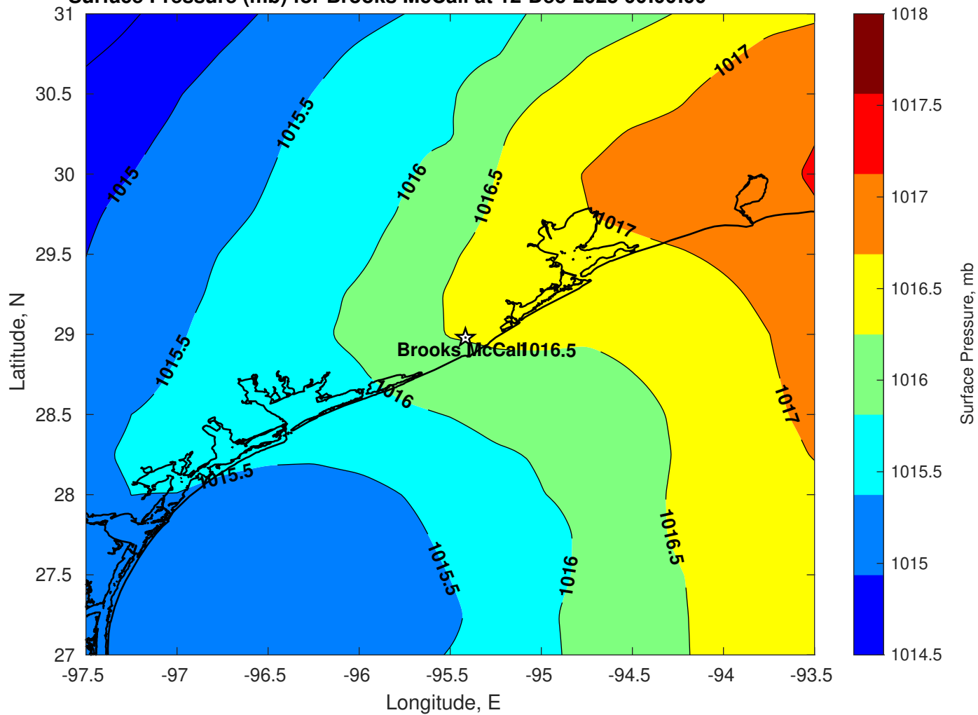
Surface Pressure (mb) for Brooks McCall at 12-Dec-2025 00:00:00
