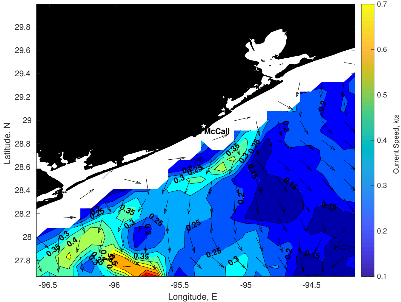
Surface Currents for Brooks McCall at 11-Dec-2025 00:00:00
