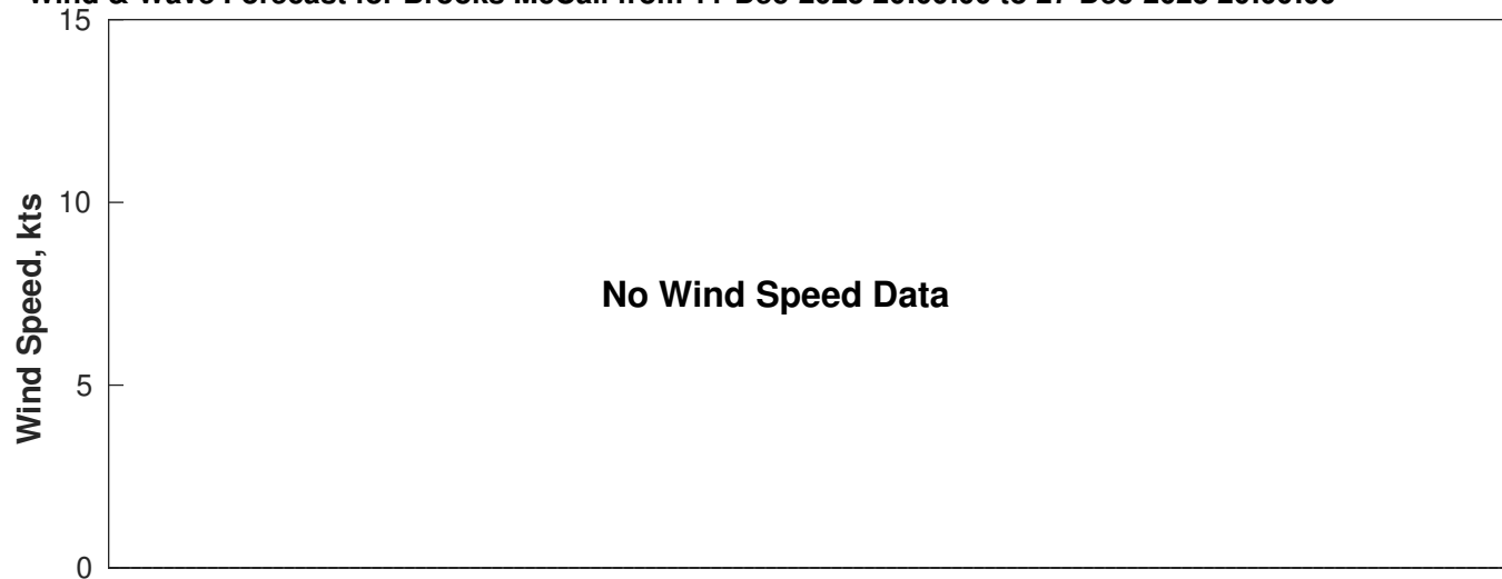
Wind & Wave Forecast for Brooks McCall from 11-Dec-2025 20:00:00 to 27-Dec-2025 20:00:00
