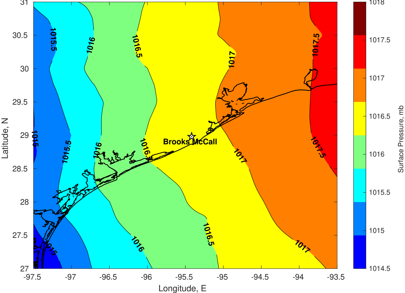
Surface Pressure (mb) for Brooks McCall at 14-Dec-2025 00:00:00
