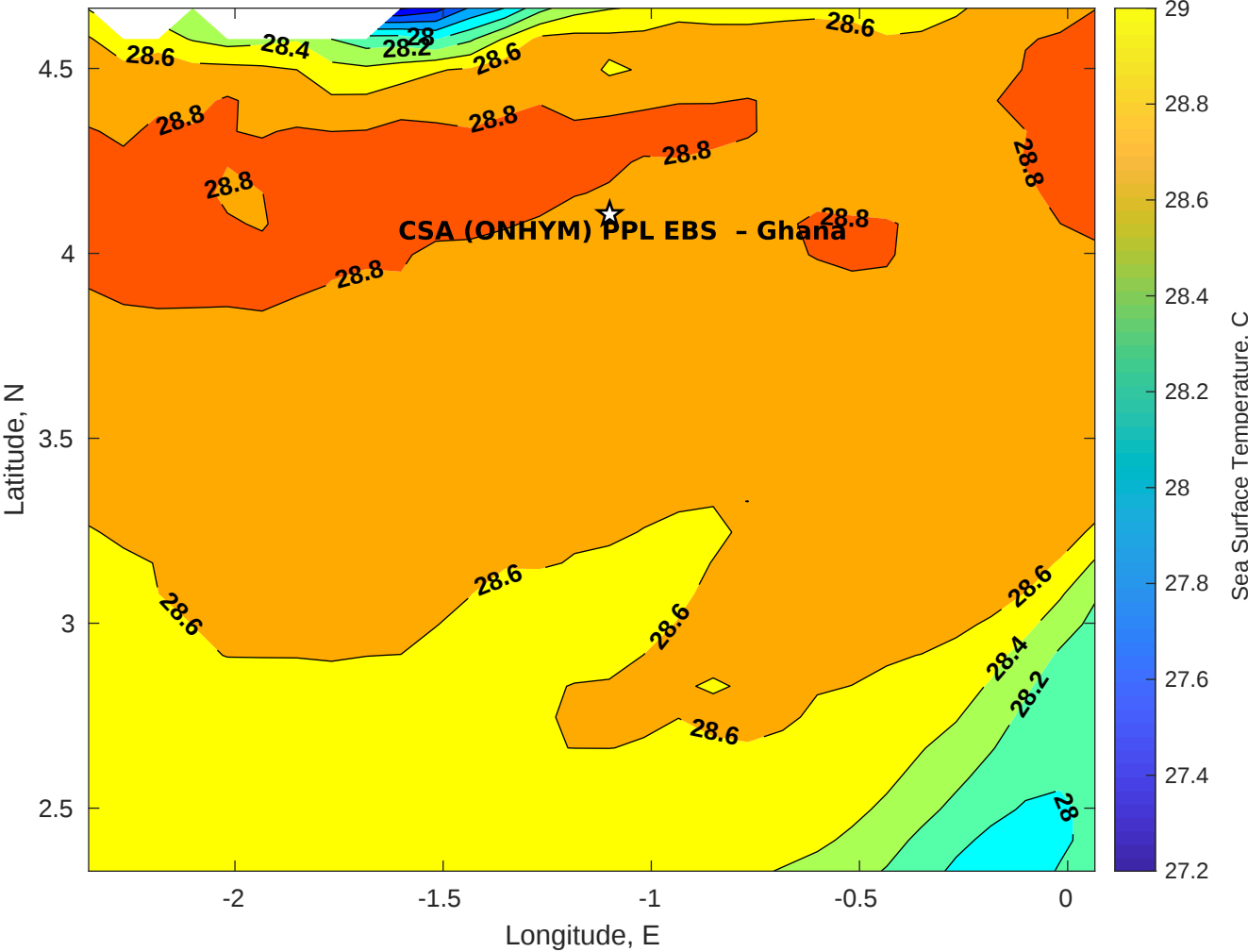
SST for CSA (ONHYM) PPL EBS - Ghana at 11-Dec-2025 00:00:00
