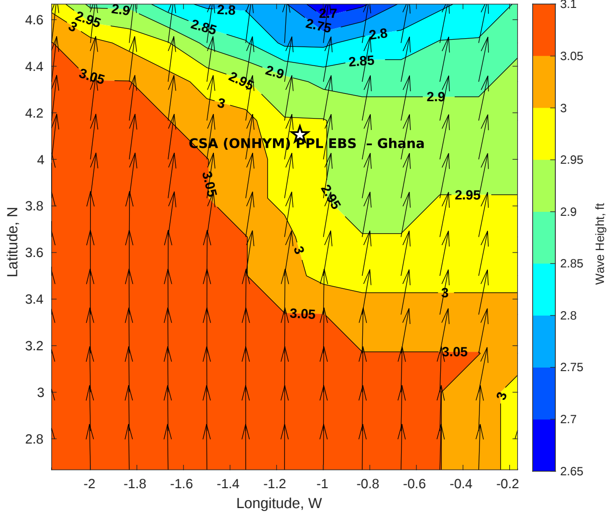
GFS Wave Height (ft) for CSA (ONHYM) PPL EBS - Ghana at 12-Dec-2025 09:00:00
