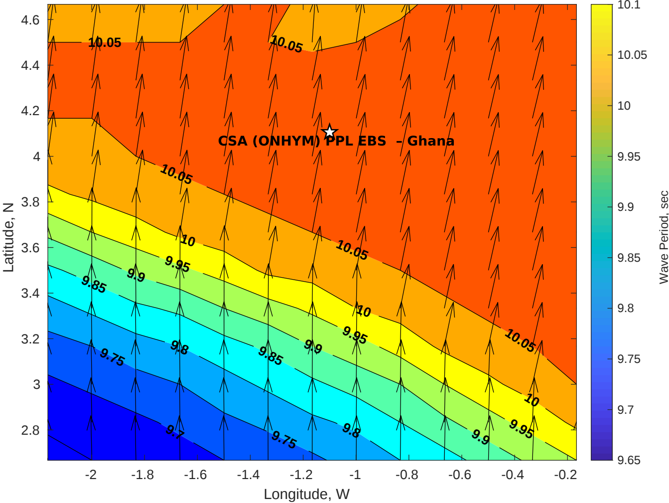
GFS Wave Period (sec) for CSA (ONHYM) PPL EBS - Ghana at 12-Dec-2025 09:00:00
