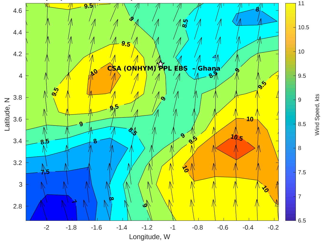
GFS Winds (kts) for CSA (ONHYM) PPL EBS - Ghana at 12-Dec-2025 09:00:00
