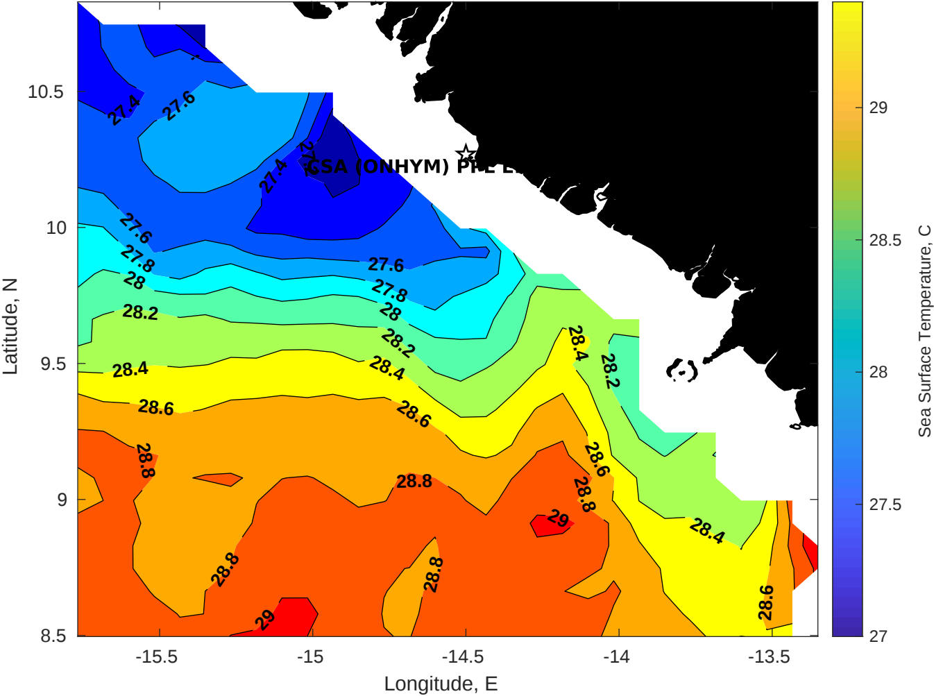
SST for CSA (ONHYM) PPL EBS - Guinea at 11-Dec-2025 00:00:00
