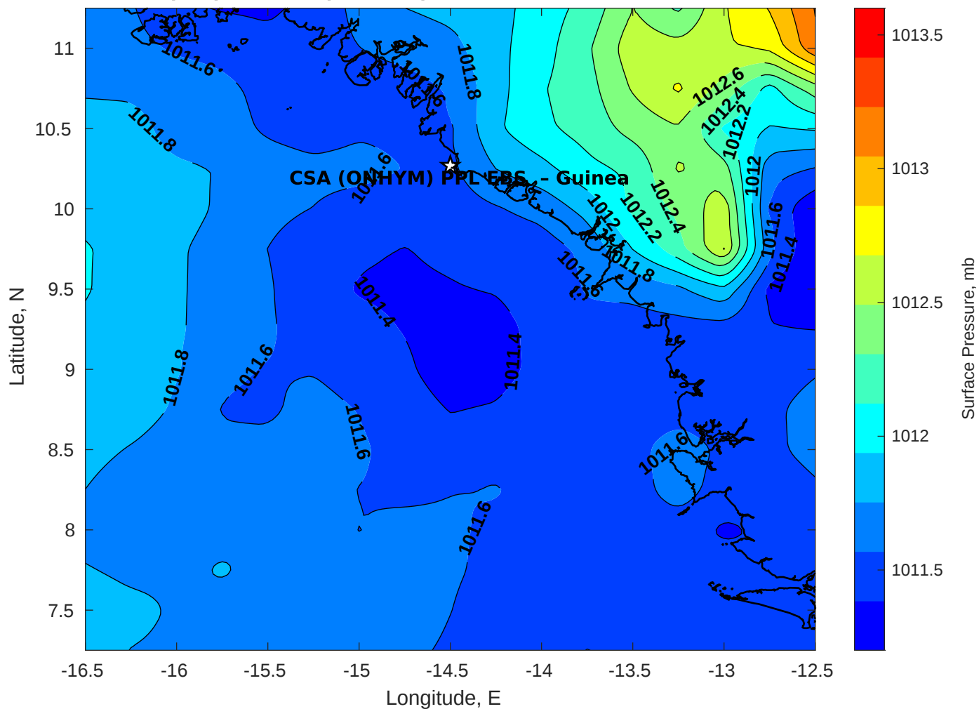
Surface Pressure (mb) for CSA (ONHYM) PPL EBS - Guinea at 14-Dec-2025 00:00:00
