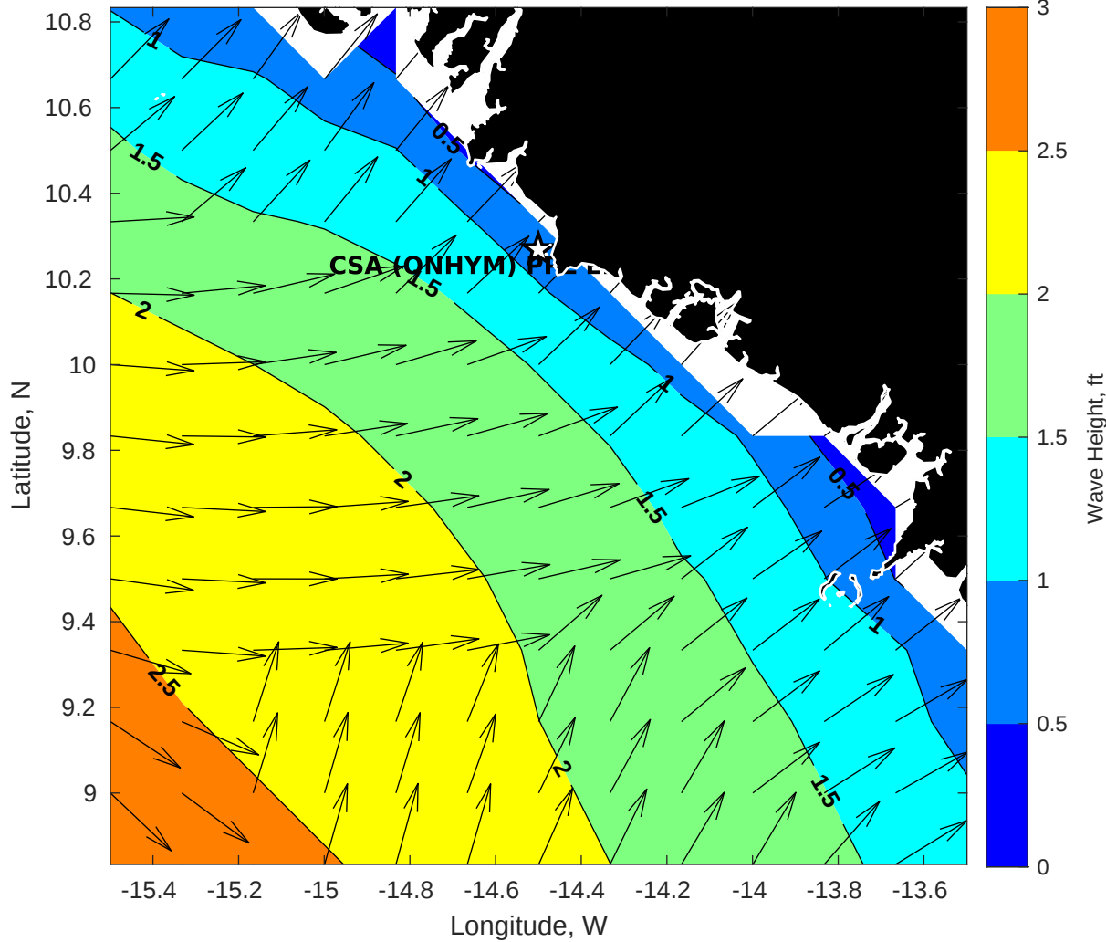
GFS Wave Height (ft) for CSA (ONHYM) PPL EBS - Guinea at 12-Dec-2025 09:00:00
